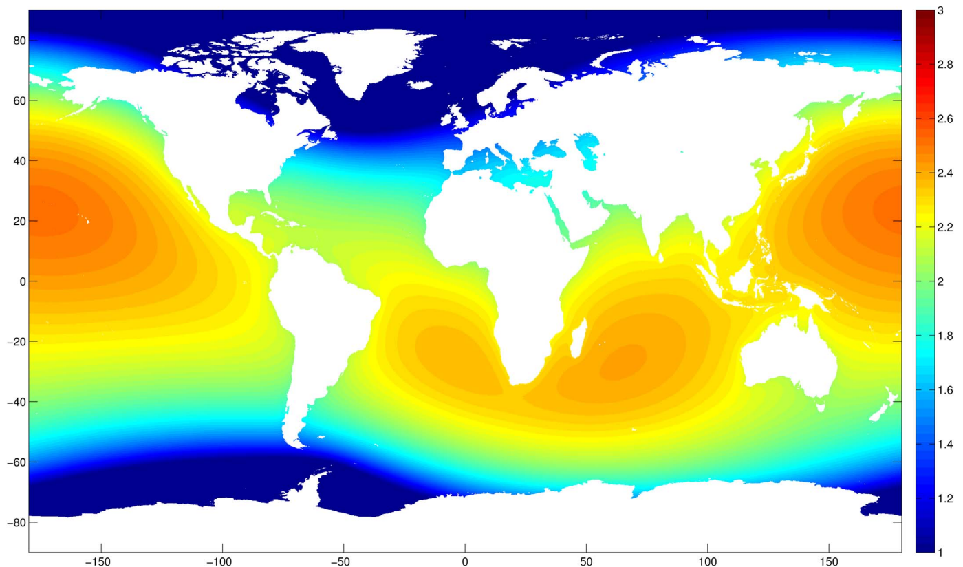
Fig. 5. The SLR perturbation (m) applied to the model for the 2 m average SLR non-uniform initial elastic response scenario with uniform ice sheet melt in both Greenland (1 m) and Western Antarctica (1 m) (+2NUB). In the near field of the areas of the mass loss sea-level change can be negative. For coastal city SLR values see Table SM1. Data courtesy of Mitrovica et al. (2001).
