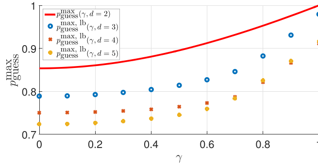
Figure 3. The optimal guessing probabilities p_{\text{guess}}^{\max}(\gamma, d) as a function of \gamma for different d . The solid line corresponds to the analytical solution p_{\text{guess}}^{\max}(\gamma, d = 2) for a two-dimensional game. The remaining data corresponds to the numerical lower bounds p_{\text{guess}}^{\max, \text{lb}}(\gamma, d) for d = 3, 4, 5 . For \gamma = 0 the numerical values coincide with the analytical solution p_{\text{guess}}^{\max}(\gamma = 0, d) = \frac{1}{2}\left(1 + \frac{1}{\sqrt{d}}\right) . The crossing of the dotted lines corresponding to d = 4 and d = 5 is discussed in section 5.
