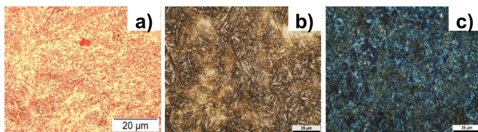
Figure 6.3: Optical microscopy of (a) initial material in the soft annealed condition, (b) sample after conventional heating rate (20 °C/s) and quenching, and (c) sample after UFHT (300 °C/s) and quenching. Etched with sodium metabisulphite.
