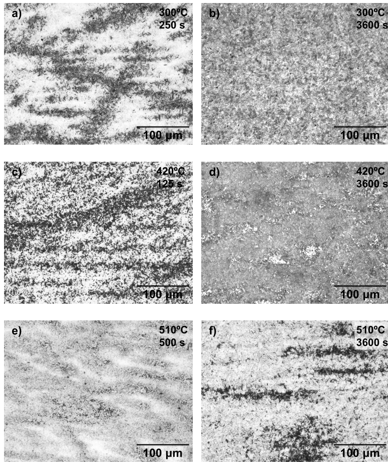
Figure 2.2: Low magnification micrographs showing the microstructure obtained after interrupted isothermal treatments, with the time and temperature indicated in the top right corner of each micrograph. In all cases, dark-etching phase is bainite and white-etching phase is fresh martensite and/or retained austenite. The samples were etched with Nital 2%.
