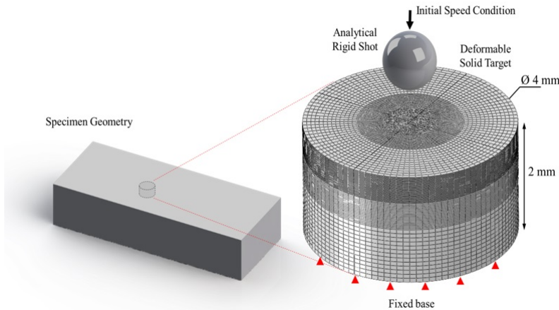
Figure 4.2: Finite Element Model of a single shot impact.
