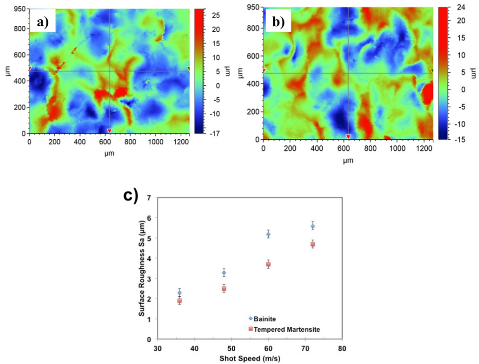
Figure 4.11: Maps of the surface roughness of the two microstructures. a) bainite, b) tempered martensite. c) Comparison of roughness values, average of 5 measurements, error bar represents the standard deviation.
