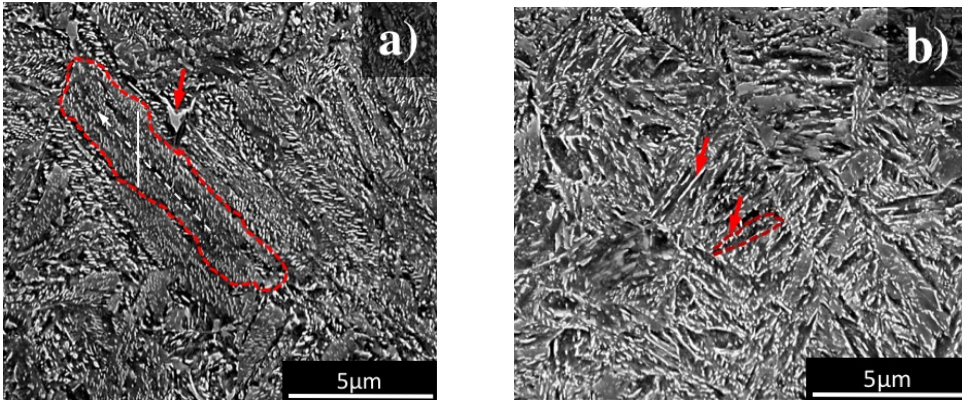
Figure 5.3: Scanning electron microscopy micrographs of the specimens with: a) bainitic microstructure, b) tempered martensitic microstructure.
