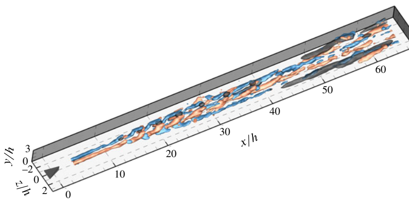
FIGURE 18. (Colour online) Instantaneous streamwise vorticity at Re_h = 460 after low-order reconstruction, perspective view; red and blue colours correspond to clockwise and anticlockwise rotation vortices, \omega_x^* = \pm 0.16 , low-speed region highlighted by black iso-surface of u'/u_\infty = -0.04 .
