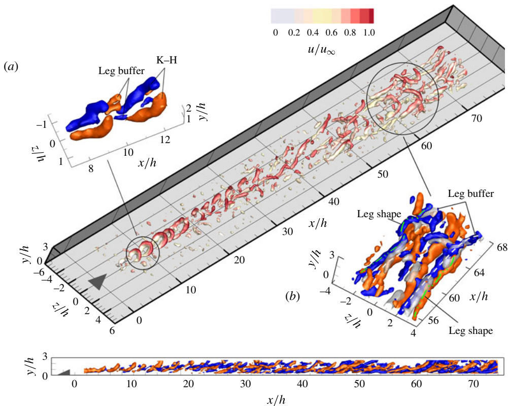
FIGURE 6. (Colour online) The instantaneous flow pattern at Re_h = 730 , perspective view detected by \lambda_2 criterion colour coded by u/u_\infty ; (a,b) and side view: streamwise vorticity, red and blue for clockwise and anticlockwise rotation vortices, \omega_x^* = \pm 0.3 ; (b) grey iso-surface: low-speed regions shown by u'/u_\infty = -0.15 , leg-buffer and leg-shaped vortices highlighted with white dashed and green dash-dotted lines.
