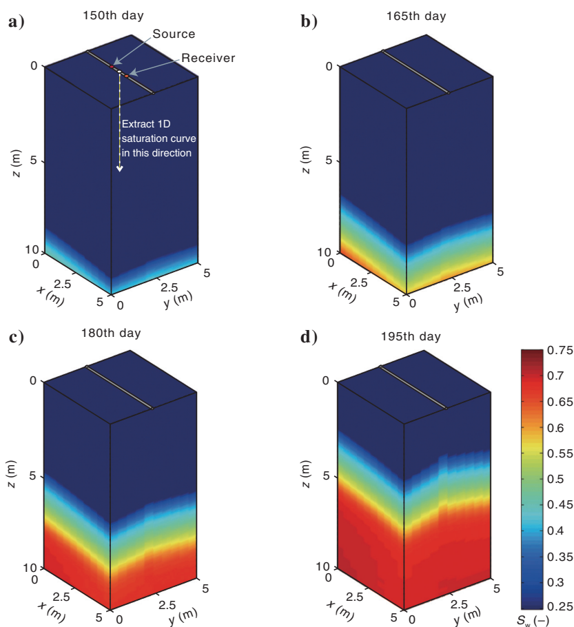
Figure 5. Snapshots of water saturation distributions in the extracted box volume on the (a) 150th day, (b) 165th day, (c) 180th day, and (d) 195th day of production, respectively. The red part represents the invading water and the blue part the oil in-place.
