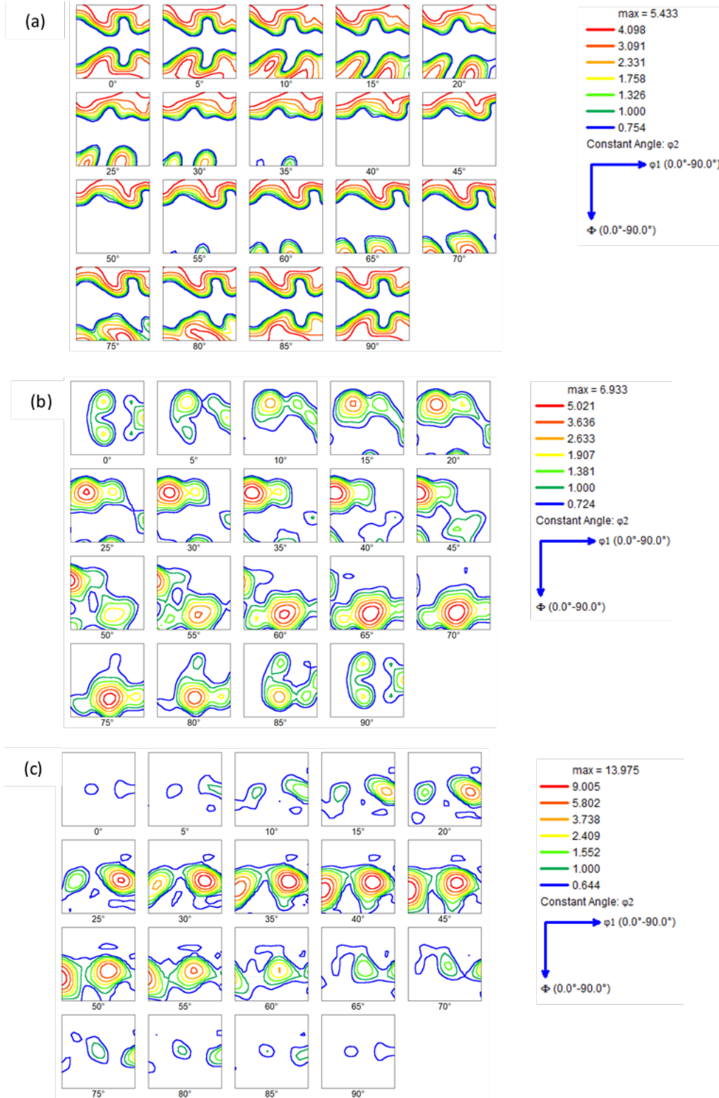
Figure 3- Orientation distribution function (ODF) plots for constant \phi_2 for samples ECAPed to 2, 6 and 10 passes in (a), (b) and (c) respectively.
