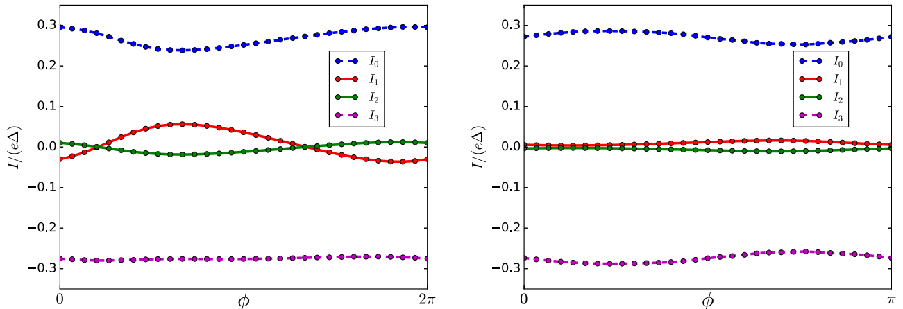
FIG. 8. Dependence of the currents on the phase shift \phi . Here \phi_0 = 2.21 , \Gamma = 0.002\Delta , and V = 0.005\Delta/e . Left: \phi_1 = eVt , \phi_2 = 3eVt + \phi . Right: \phi_1 = 2eVt , \phi_2 = 3eVt + \phi . We see that already 10 phase shifts give a rather good sampling.
