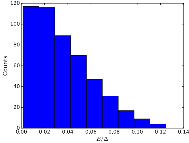
FIG. 7. To observe the quantization of the transconductance, it is favorable to have (\phi_1, \phi_2) planes with a large spectral gap both in the topological and the trivial region. Here we show a histogram of the smaller of the maximal gaps in these two regions for 500 random scattering matrices with Weyl points.
