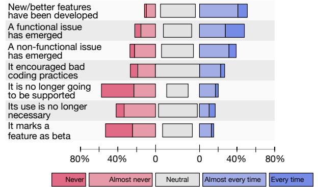
Figure 3: Motivations to react to deprecation according to API consumers' experience, by decreasing frequency
