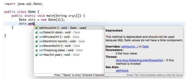
Figure 1: Example of deprecation warning in the IDE
