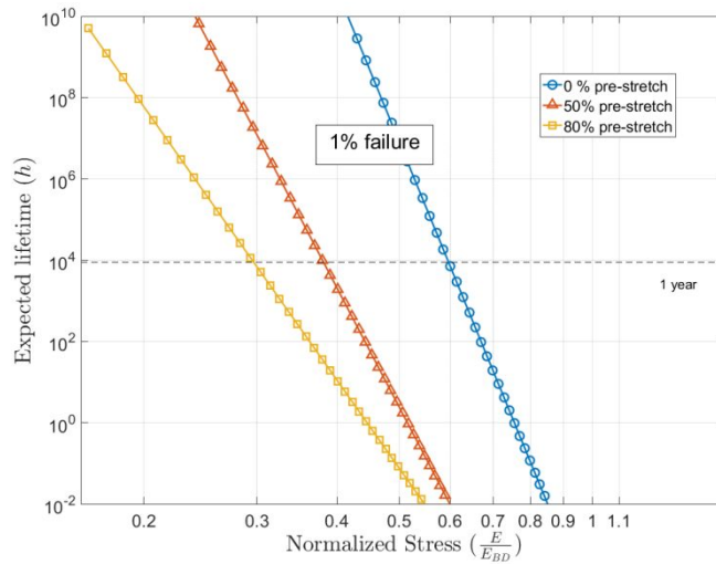
Figure 6. 1% Failure curves for the three membrane set. For better comparison, the stress has been normalized to respective breakdown field.
