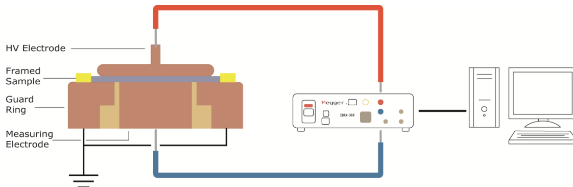
Figure 1. Dielectric spectroscopy setup. Measuring cell is depicted on the left-side. Top electrode, guard ring and bottom electrode are brass-made. The insulation between the guard ring and the measuring bottom electrode is epoxy-based. The scale is exaggerated for readability purpose.
