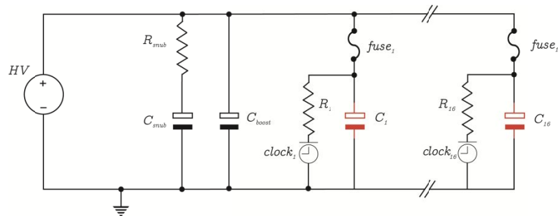
Figure 5. Parallel DC lifetime setup schematics with a single high voltage DC source. The sample-under-test C_i disconnection from main line at breakdown event is done through corresponding fuse fuse_i blowing. At the same time, corresponding timer clock_i stops counting. Up to 16 samples can be tested at the same time with this setup. Timer resolution is 0.01 h. For this work, HV source used is Heinzinger PNC1000-15.
