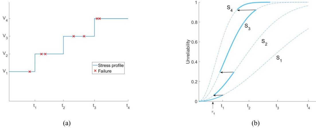
Figure 3. (a) Step-stress example pattern over time and (b) resulting cumulative Weibull cdf.
