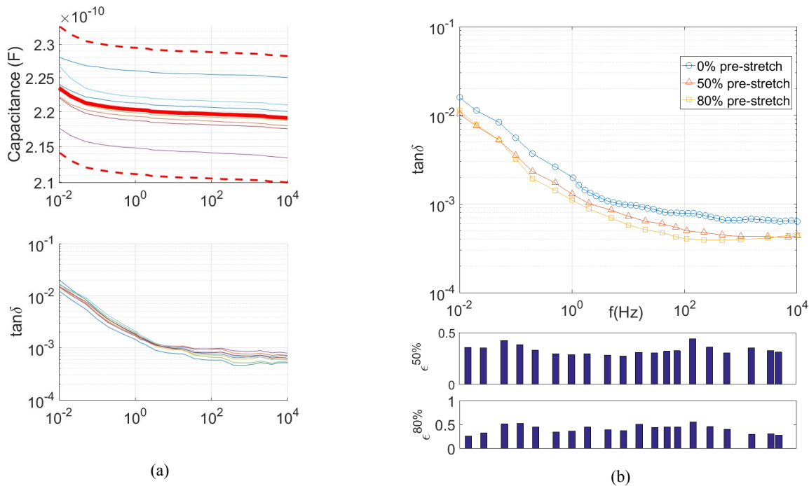
Figure 2. (a) Top Capacitance spectrum for specimen set 1. Thick line represent is the average value, dashed line the rejection bounds. Bottom: \tan\delta for the same set. (b) Top: average \tan\delta measurements for each membranes set. Bottom: absolute value of the relative difference by \tan\delta of non-stretched membrane and the 50% and 80% stretched ones, respectively.
