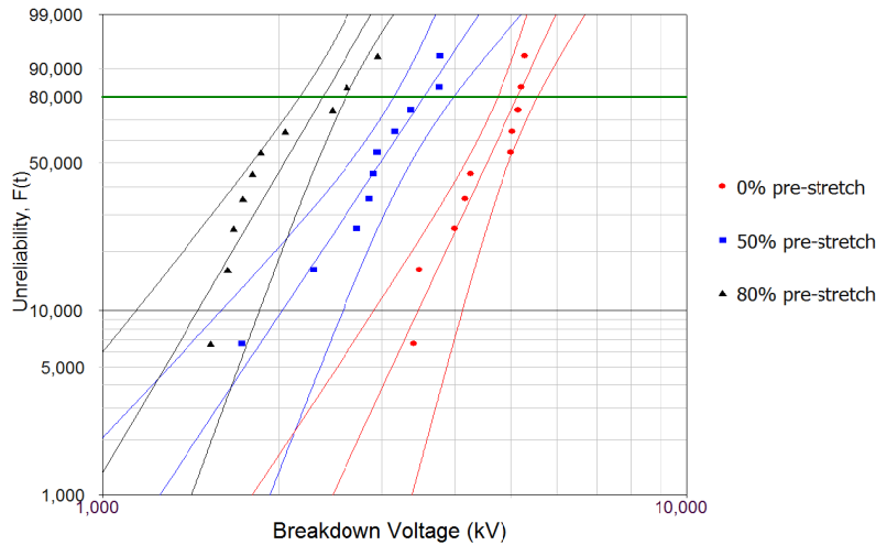
Figure 4 Weibull plot corresponding to preliminary breakdown voltage characterization of the three available set. Specimens with higher stretch and, thus, thinner, have lower breakdown voltage. The test was executed by ramp voltage on 10 different specimen for each stretch set.
