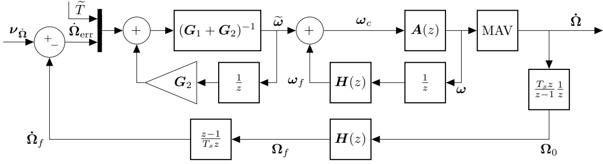
Figure 3: The inner INDI control structure.
