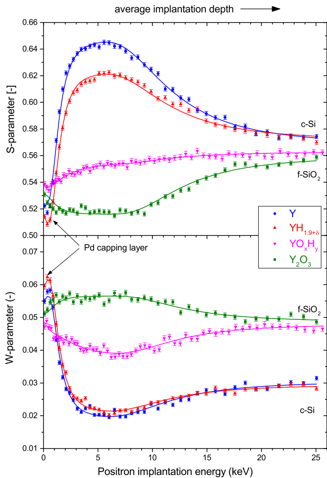
Fig. 2. Doppler Broadening PAS S and W depth profiles of Y, \text{YH}_{1.9+\delta} , \text{YO}_x\text{H}_y and \text{Y}_2\text{O}_3 thin films on f-SiO 2 or c-Si substrates. The full curves are best-fits obtained using VEPFIT analysis.
