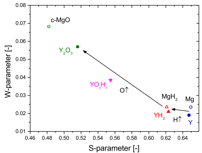
Fig. 3. S-W diagram of the S and W best-fit values for the Y, \text{YH}_{1.9+\delta} , \text{YO}_x\text{H}_y and \text{Y}_2\text{O}_3 thin films. For comparison, the S-W points for Mg and \text{MgH}_2 [19,21] thin films and c-MgO [32] are included. The arrows labeled by H↑ and O↑ indicate the trends upon increased hydrogen and oxygen insertion, respectively.
