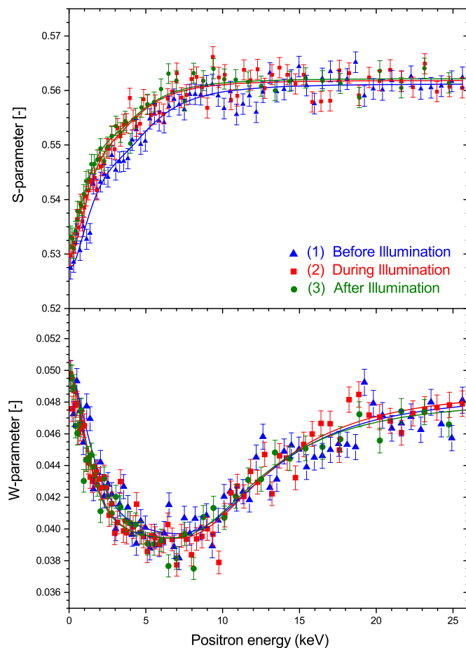
Fig. 6. S and W depth profiles of photochromic \text{YO}_x\text{H}_y sample #1 on \text{f-SiO}_2 substrate as a function of positron implantation energy before UV illumination (1), at the end of the illumination with the UV-lamp still switched on (2), and after 48 h of bleaching under dark conditions (3).
