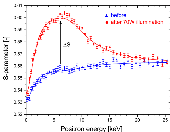
Fig. 9. Doppler S parameter depth profiles before and after the 1.5 h heat treatment at 130 °C (70 W).
