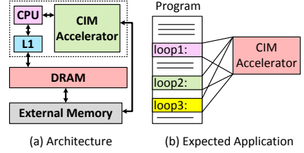
Fig. 9: CIM-based Architecture
