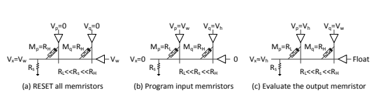
Fig. 4: Stateful Logic
