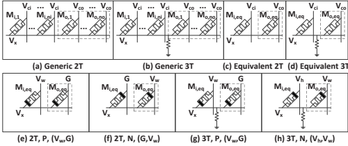
Fig. 3: 2T and 3T Logic Gates.
