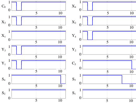
Fig. 15: Waveform of OD Adder SPICE Simulation.
