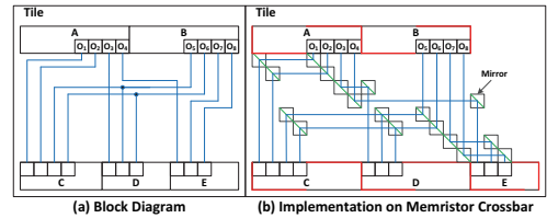
Fig. 9: General Intra-Tile Interconnect Network Using Mirrors
