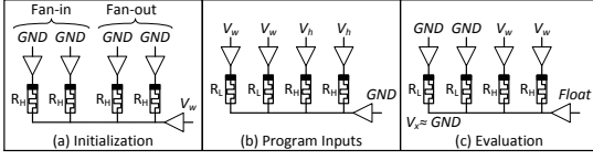
Fig. 3: An Example of an AND Gate
