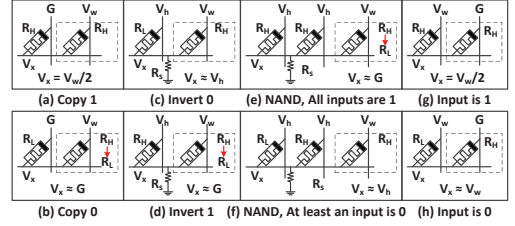
Fig. 2: Basic Operations
