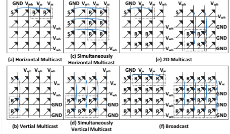
Fig. 5: Multicast and Broadcast Communication Schemes
