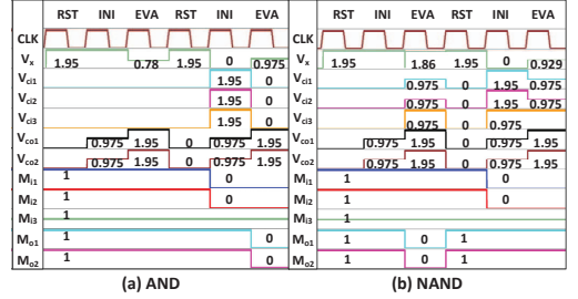
Fig. 6: Simulation Results of Logic Gates.
