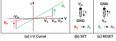
Fig. 1: Memristor model [9].
