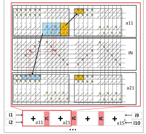
Fig. 6: Memristor-based Interconnect Network
