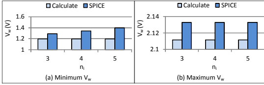
Fig. 7: Impact of Nanowire Resistance
