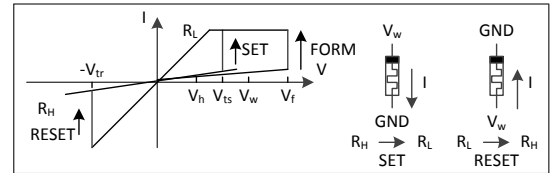
Fig. 1: Behaviour of a Memristor [9].
