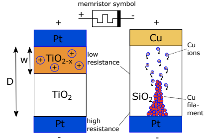
Fig. 5: ECM (left) and VCM (right) ReRAMs (ECM).
