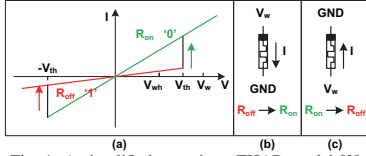
Fig. 1: A simplified memristor THAB model [3].
