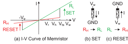
Fig. 1: Memristive Behaviour.
