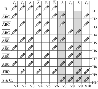
Fig. 10: The FA Calculating All Outputs Simultaneously.
