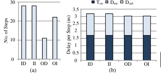
Fig. 17: Delay of Selected Designs: (a) Number of Execution Steps, (b) Delay per Execution Step.
