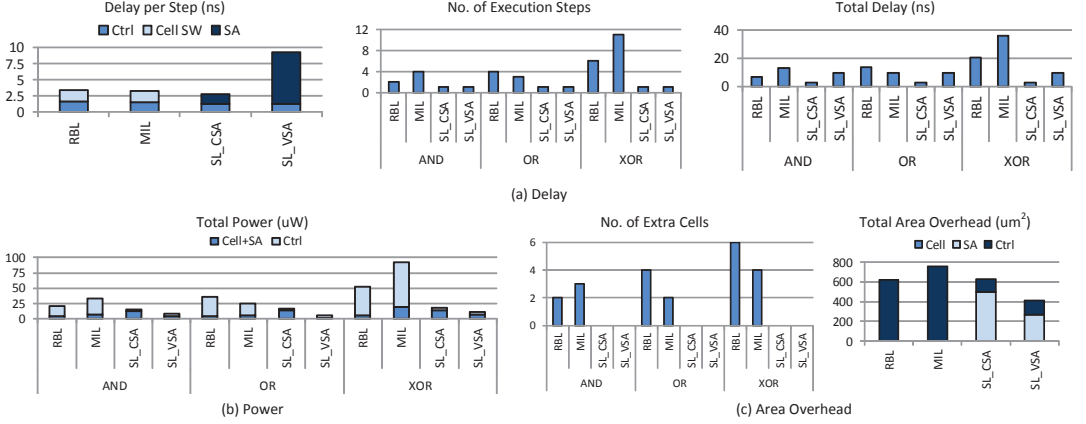
Fig. 8: Comparison Between Different Logic Styles
