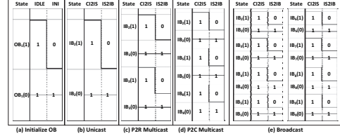
Fig. 13: Simulation Results of 2D Bus
