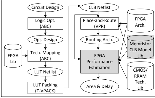
Fig. 7: A CAD Flow for MFPGA and RFPGA
