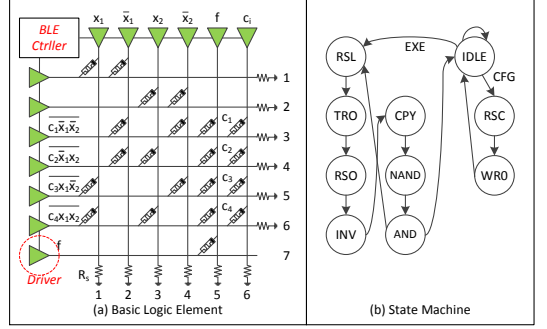
Fig. 6: RFPGA
