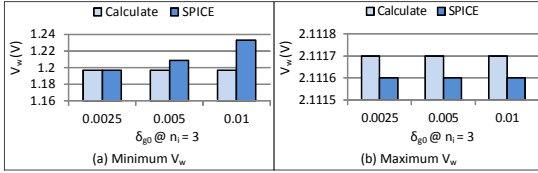
Fig. 6: Impact of Device Variation
