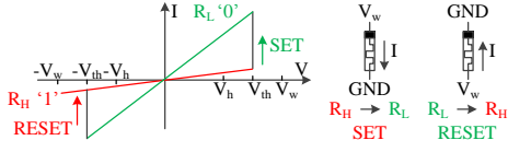
Fig. 1: Ideal Memristor Model.
