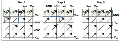
Fig. 7: Multi-Bit Communication with Mirrors
