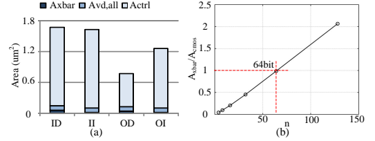
Fig. 16: Area of Selected Designs: (a) Area, (b) Scalability Exploration.
