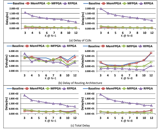
Fig. 12: Delay of Different FPGAs
