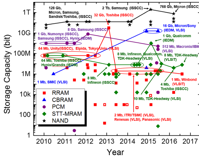
Figure 1.3: Trends of Emerging Device Technologies [18]
