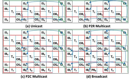
Fig. 11: 2D Bus Communication Schemes
