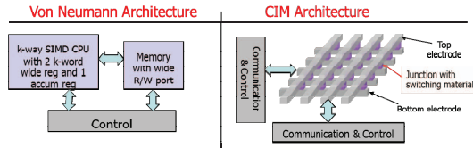
Figure 2: Traditional versus proposed architecture
