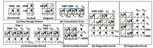
Fig. 6: Multi-Bit Word Storage Patterns and Communication
