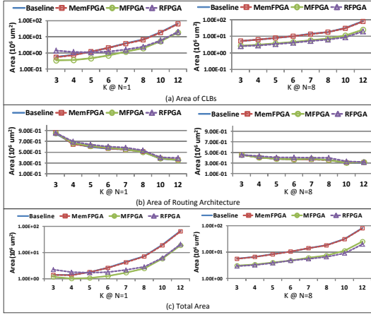
Fig. 11: Area of Different FPGAs
