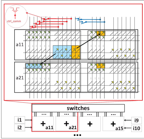
Fig. 7: Hybrid Interconnect Network
