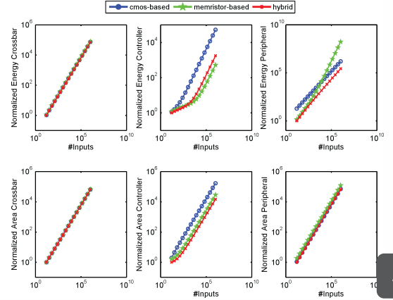
Fig. 10: Performance Breakdown of Each Component
