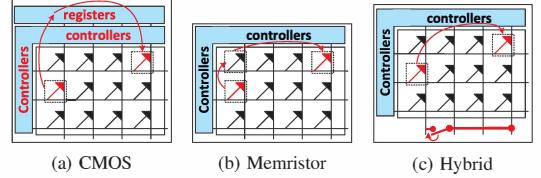
Fig. 4: Proposed Interconnect Network
