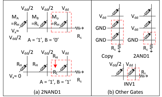
Fig. 3: Logic Gates of Resistive Boolean Logic
