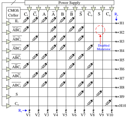
Fig. 4: Implementation of One-Bit Full Adder.
