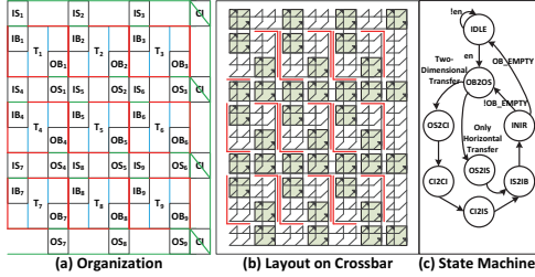
Fig. 10: 2D Bus General Inter-Tile Interconnect Network
