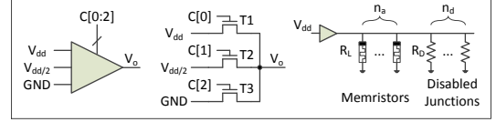
Fig. 9: CMOS Voltage Drivers.
