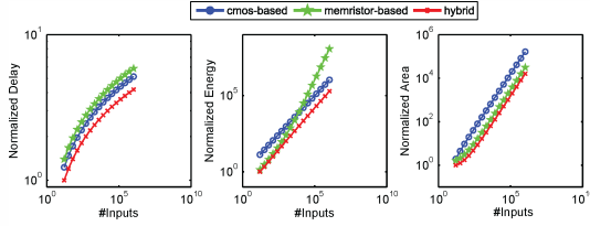
Fig. 9: Performance of Proposed Interconnect Network Schemes
