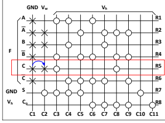
Fig. 5: Example of Sneak Path Currents for a One-Bit Full Adder
