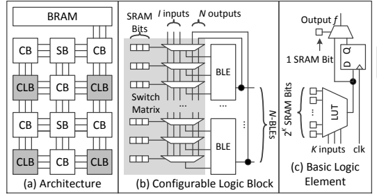
Fig. 4: Island-Style FPGA Architecture
