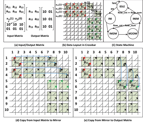
Fig. 8: Matrix Transpose on Memristor Crossbar
