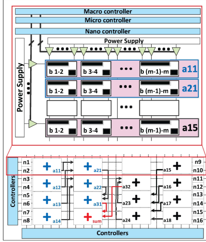
Fig. 2: CIM-based Parallel Adder (16 inputs)
