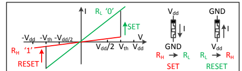
Fig. 1: Electronic Characteristics of Memristor
