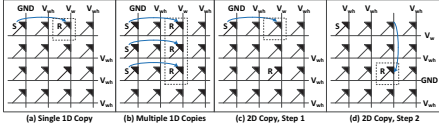
Fig. 4: Unicast Communication Schemes
