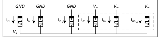
Fig. 4: Generic AND Gate in Evaluation Step
