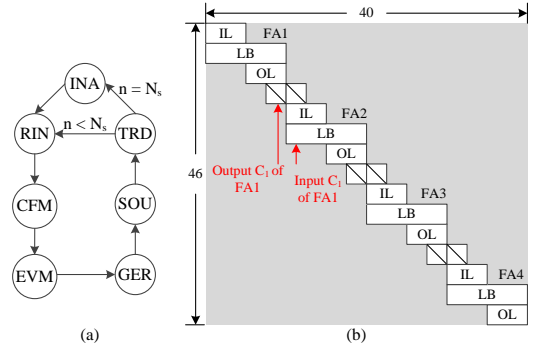
Fig. 11: Diagonally-Mapped Adder: (a) State Machine, (b) Layout.
