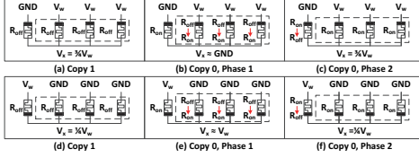
Fig. 3: Multi-Fanout Copy Operation
