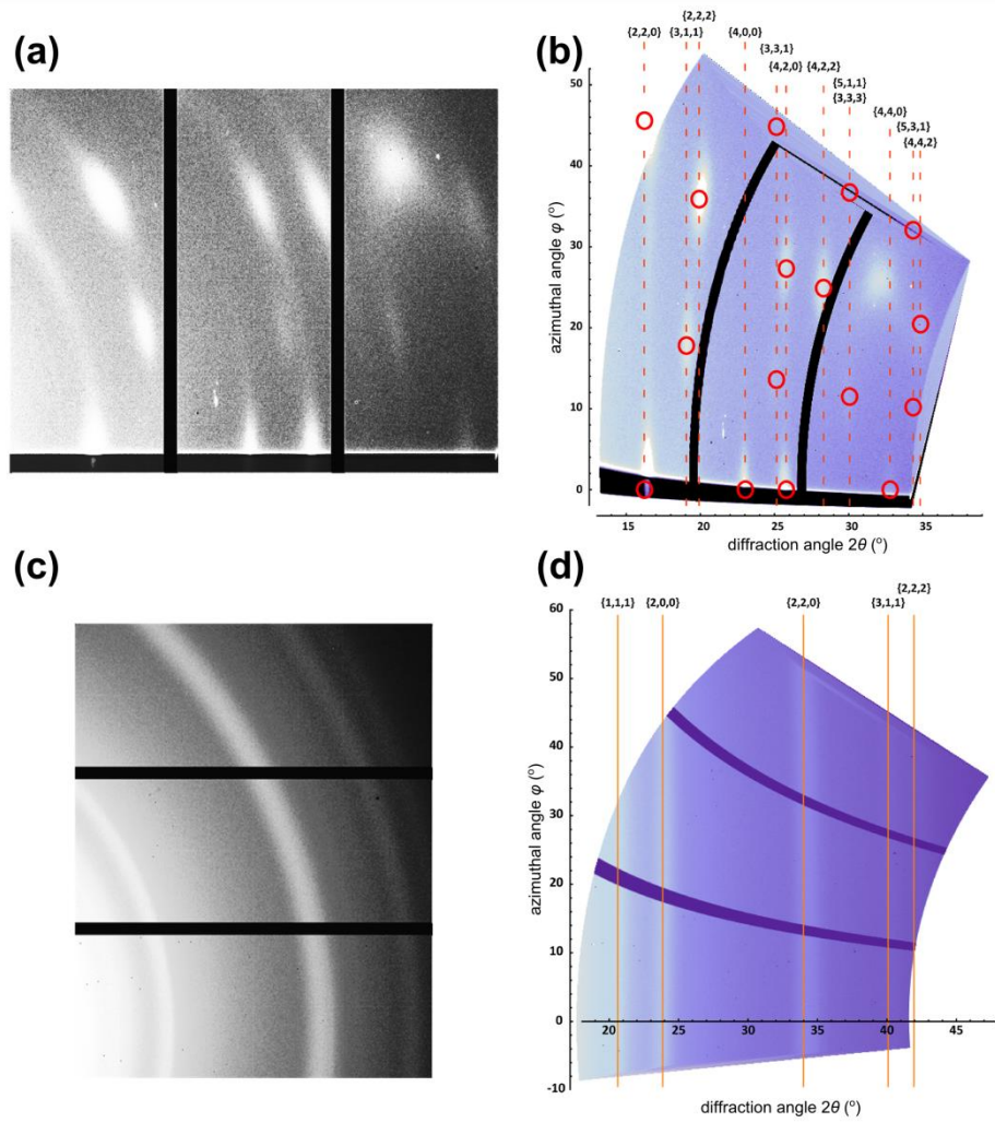
Figure S18: GIWAXS parametrization and data analysis. (a) Atomically aligned NCs on top of a Si-(100) substrate with their [100] axis perpendicular to the surface, giving rise to diffraction spots on the GIWAXS detector. (b) Same image, after coordinate transformation from pixel values to 2\theta and \phi values. The red dots are the positions of the expected atomic reflections. The only unlabeled diffraction peak at (2\theta, \phi) = (32^\circ, 28^\circ) corresponds to a Si reflection, the sample substrate. These GIWAXS patterns were recorded during initial experiments at an X-ray energy of 20.7 keV. (c) GIWAXS of the PbSe NCs in solution. These are identical particles to those used for the in-situ experiments in the main text. (d) Transformed GIWAXS image, showing the position of the diffraction rings. Experiments recorded with the same experimental parameters as the in-situ experiments.
