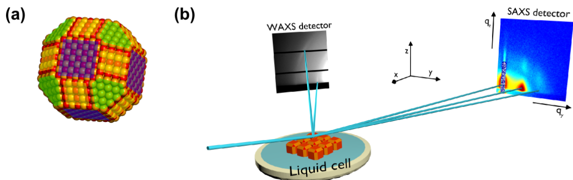
Figure S1: Schematic of the in-situ GISAXS/GIWAXS study of nanocrystal assembly at the liquid/air interface. (a) An atomic model of the PbSe truncated nanocubes, showing the different facets of the NC. Blue indicates the {100} facets, yellow the {110} facets and green the {111} facets. (b) Schematic of the setup used for in-situ GISAXS/WAXS experiments. A dispersion of NCs in toluene evaporates in a liquid sample cell. We examine the process of assembly and attachment using grazing-incidence x-ray scattering, by simultaneously monitoring the atomic order on the wide-angle detector and nanoscale order on the small-angle detector.
