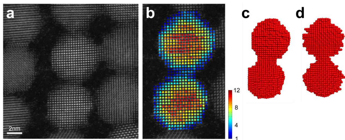
Figure S23: HAADF-STEM and atom counting reconstruction on attached NCs. (a) HAADF-STEM image of NCs attached in a square superlattice. The atomic periodicity is continued from a given NC to its neighbors. Slight misorientations can also be observed. (b) Results from the atom counting procedure, using (a) as an input image. The color bar represents the number of detected atoms in each vertical column. (c) Top-view and (d) side-view of the reconstructed atomic model.
