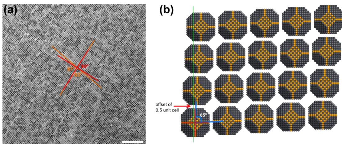
Figure S8: Discussion on the bond-angles in the final square superlattices. Due to the crystal structure of the individual PbSe nanocrystals, a shift of 0.5 unit cells in the two lateral directions is required to result in Pb-to-Se binding. The resulting bond angles would then be slightly larger or slightly smaller than 90^\circ . (a) TEM image of a superlattice, where the deviation of the bond angles ( 83^\circ/97^\circ ) with a perfect square lattice ( 90^\circ ) is clearly seen over longer distances. (b) Models of the PbSe nanocrystals in a square superlattice, where in both lateral directions the particles are shifted by half a unit cell. The scale bar in the TEM image equals 100 nm.
