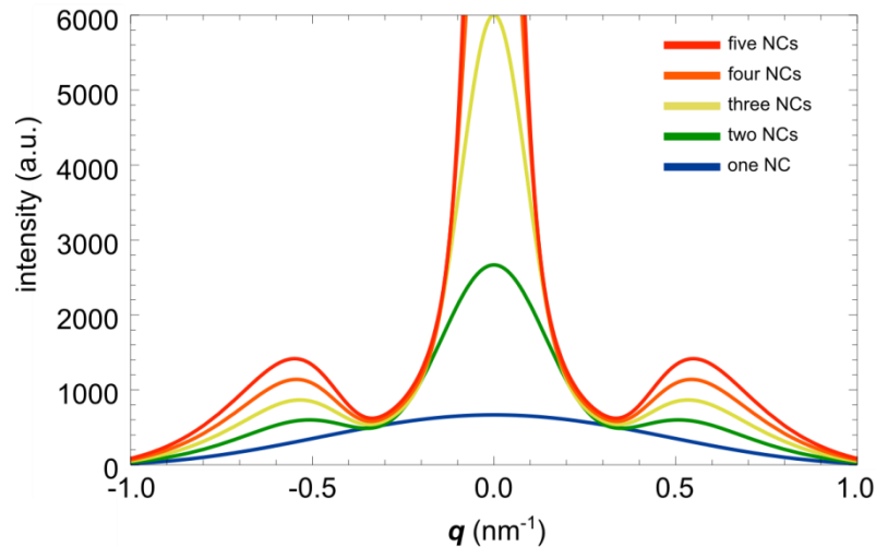
Figure S20: peak width of aligned but not connected nanocrystal as a function of increasing number of attached nanocrystals. Plotted are the scattering curves using d = 0.6 nm, N = 9 (the product N \cdot d gives a realistic nanocrystal size), L_0 = 1.53 \cdot N \cdot d . We used \sigma L = 0.4 \cdot L_0 .
