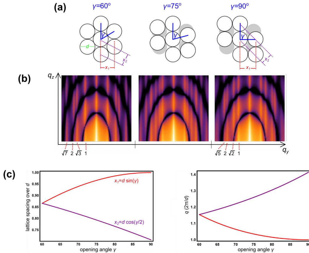
Figure S17: Simulated GISAXS pattern as function of bond angles. (a) The three models which were calculated: a 2-D hexagonal crystal, a 2-D crystal with a bond angle of 75^\circ and a 2-D square crystal. The lattice planes that are equivalent in the hexagonal crystal ( x_1 and x_2 ) break their degeneracy when the bond angle is changed from 60^\circ to 90^\circ . Here, d equals the diameter of the spheres. (b) Calculated GISAXS patterns for the corresponding 2-D crystals. Note how all diffraction rods split when the opening angle is 75^\circ . Also note that for the 2-D square crystal the first higher order diffraction rod (indicated with \sqrt{2} ) coincides precisely with the first form-factor minimum at low values of q_z . (c) The change of the relative lattice spacings x_1 and x_2 over d , when going from the 2-D hexagonal crystal to the 2-D square crystal in direct space (left) and reciprocal space (right). Note how the degeneracy is lifted when the bond angle differs from 60^\circ .
