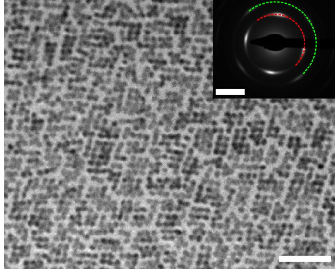
Figure S5: Characteristic TEM image of the sample scooped from the surface used in the in-situ experiments shown in Fig. 2 of the main text. Note the resemblance to Fig. 2(g). The micrograph shows that the NCs have assembled into a square superlattice. The NCs are atomically attached only in relatively small separate patches of 10-30 NCs, which could explain the peak broadening and absence of higher order diffraction rods in the GISAXS patterns. The electron diffraction pattern shows diffraction arcs, indicating atomic alignment of the particles. The coloured rings index the diffraction spots: red = {200} and green = {220}. Scalebars denote 50 nm in the TEM image and 20 \text{ nm}^{-1} in the diffraction pattern. We should remark here that the formation of rather small domains that are atomically aligned has to do with the conditions under which in-situ measurements are done. Under better controlled conditions \mu\text{m} -large atomically coherent domains are observed (see e.g. figures S8).
