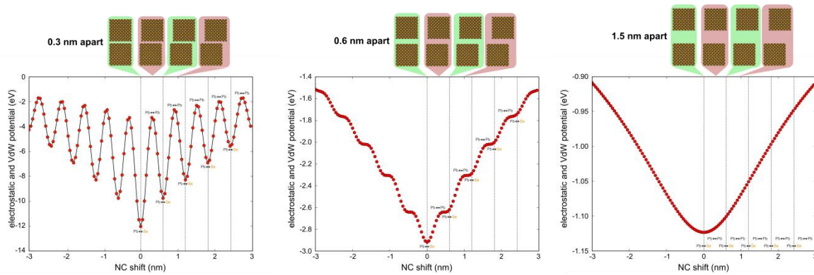
Figure S24: The interaction between two nanocubes of PbSe upon lateral displacement. The left, middle and right images shows the interaction potential when the nanocrystals are 0.3 nm, 0.6 nm and 1.5 nm apart respectively.
