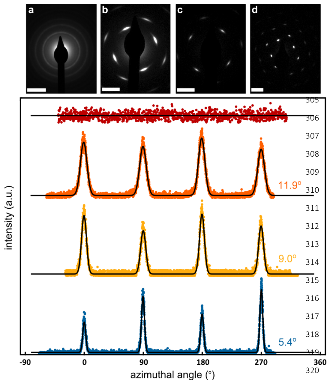
Figure S21: azimuthal peak widths of the electron diffraction patterns during the self-assembly process. ED patterns and azimuthal azimuthal traces over the {400} reflection show a decrease in peak width, which indicates the loss of in-plane rotational freedom of the nanocrystals during the self-assembly process.
