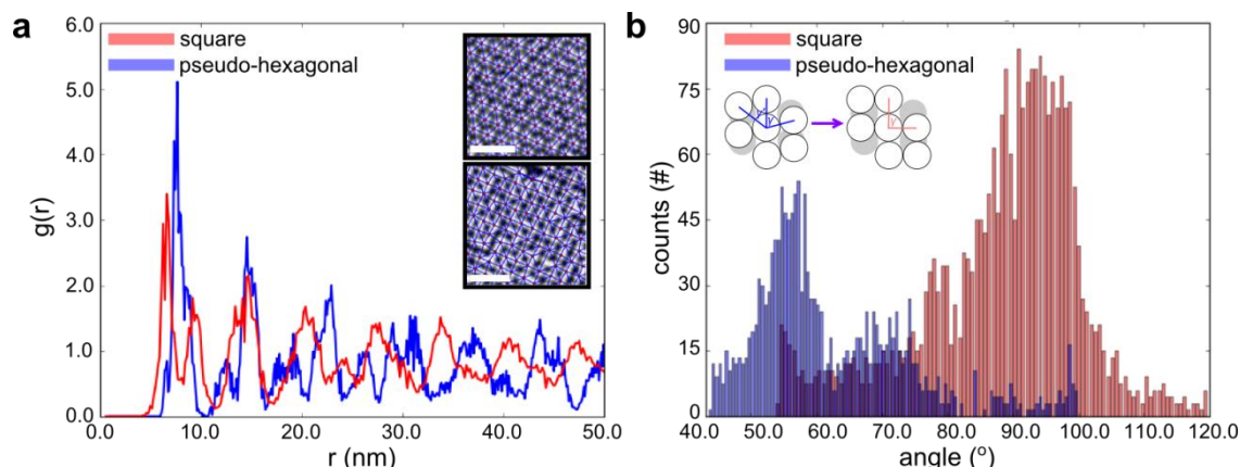
Figure S16: Image analysis on the PH and square phase TEM images. (a) Pair distribution function obtained from the detected centers of mass of the PH phase (blue) and square phase (red). The large number of oscillations is a signature of extended positional order in the superlattice. The insets show the detected particles with the Delaunay triangulation mesh for the PH (top) and square (bottom) phase. (b) Bond angles of the superlattice in the PH (blue) and square phases (red). The inset shows a schematic of the two phases displayed on top of a perfect hexagonal crystal (grey dots). Scale bars in the TEM inset are 25 nm.
