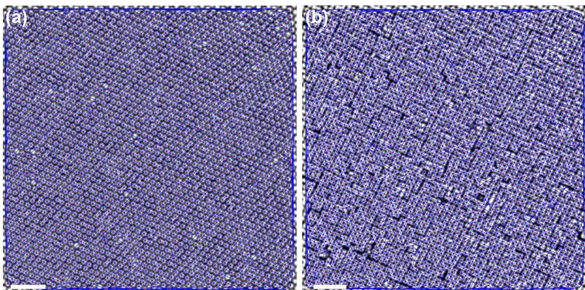
Figure S14: Computer aided image analysis on the TEM images. (a) The pseudo-hexagonal phase and (b), the square phase. The red dots indicate the centers of mass, the blue mesh is the Delaunay triangulation over these centers of mass.
