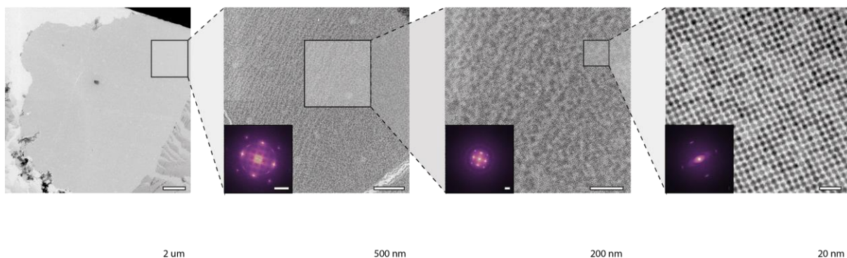
Figure S22: Conservation of nanocrystalline order on mesoscopic length scales. From left to right consecutive zoomed in TEM images are displayed, which show a very long-range periodicity. Even though the atomic coherency throughout the complete lattice is conserved over several nanocrystals, this does not perturb the long-range nano-crystalline order. From the widths of the {100}-superlattice reflections in the Fourier transforms we obtain nanocrystal coherence lengths for the superlattice of 39.3 nm, 34.3 nm and 35.9 nm from left to right. Scale bars from left to right images are 2 \mu\text{m} , 500 nm, 200 nm and 20 nm respectively and 1 \text{nm}^{-1} for all Fourier transform insets.
