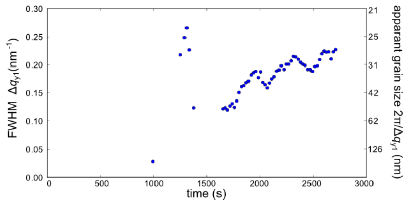
Figure S6: Analysis of the peak width of the first diffraction rod in the horizontal scattering direction \Delta q_{y1} during the GISAXS experiments shown in Fig. 2 of the main text. The grain size is calculated as 2\pi/\Delta q_{y1} , which corresponds to the Scherrer equation with K=1 if you realize that \Delta q = 4\pi/\lambda \cos(\theta) \Delta(2\theta)/2 . To reduce X-ray beam damage on the sample we scanned the sample perpendicular to the incoming X-ray beam over an area of 4 mm. The peak widths are likely to come from superlattice grains on the sample with slightly different sizes.
