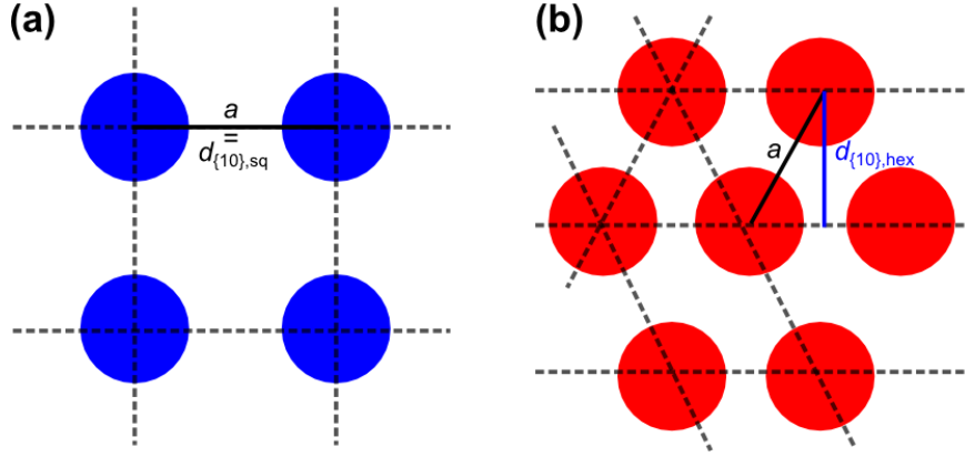
Figure S3: Origin of the first diffraction rod in GISAXS and its relationship to the NC-NC distance. (a) In the case of square ordered superlattices, the NC-NC distance a is equal to the d -spacing of the first lattice plane d_{\{10\},sq} . The corresponding q -vector is q_{\{10\},sq} = 2\pi/d_{\{10\},sq} = 2\pi/a . (b) For an hexagonal monolayer of NCs, the lattice spacing is not equal to the NC-NC distance; d_{\{10\},hex} = \sqrt{3}a/2 . The corresponding q -vector then equals q_{\{10\},hex} = 2\pi/d_{\{10\},hex} = 4\pi/(\sqrt{3}a) . Comparing the square and hexagonal lattices, the q -vector relationship for the first diffraction is different by a term 2/\sqrt{3} . In general the position of any GISAXS reflection in the horizontal scattering direction q_y with miller indices \{h,k\} for a square lattice is equal to q_{\{h,k\},sq} = \frac{2\pi}{a}\sqrt{h^2 + k^2} , while for an 2-D hexagonal lattice it equals
