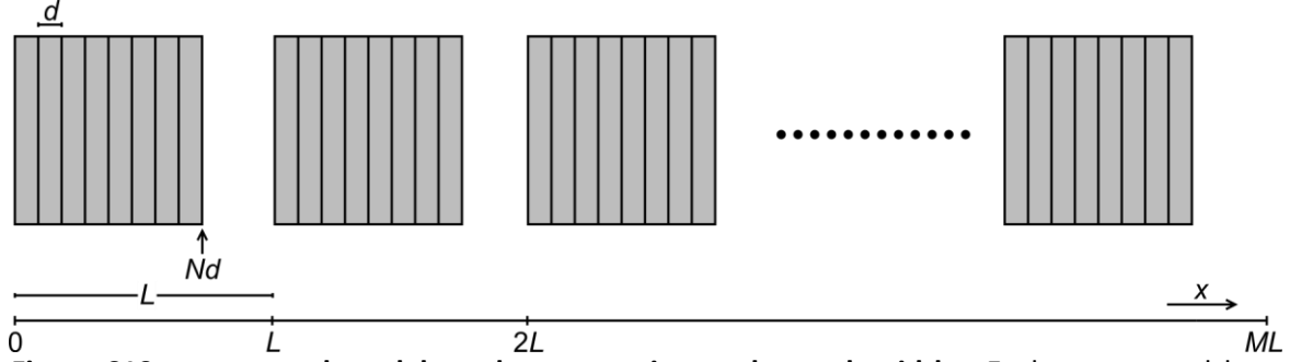
Figure S19: nanocrystal model used to approximate the peak widths. Each nanocrystal has a N lattice planes with a lattice spacing d . The length from the start of the NC to its neighbour equals L .
