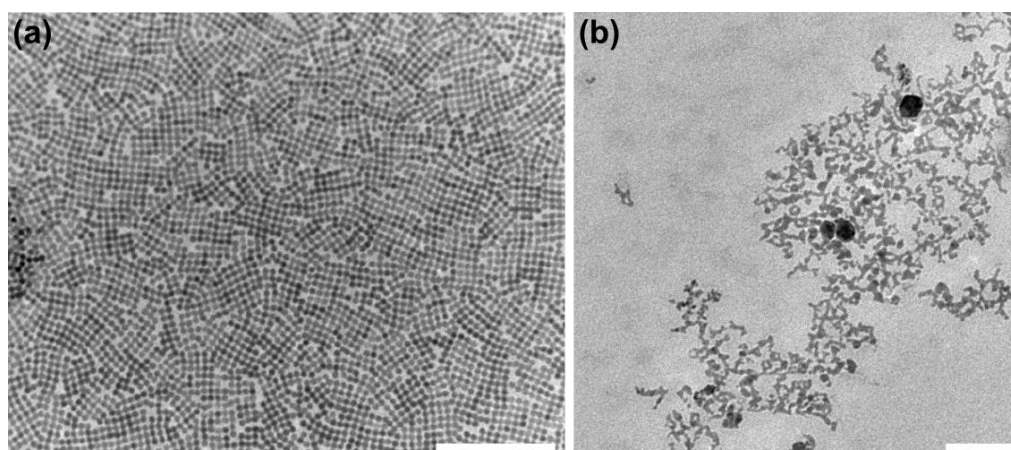
Figure S2: Diffusion limited attachment of PbSe NCs results in structures with no long-range nanoperiodic nor atomic order. (a) Sample where a large amount of simultaneous nucleation has taken place resulting in small domains with square geometry. (b) Sintered structures, with no long-range nanoperiodic or atomic order. Scale bars equal 100 nm.
