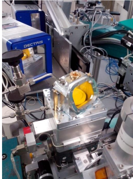
Figure S10: Photograph of the home-built liquid cell and setup used for the in-situ GISAXS/WAXS experiments at ID10 of the European Synchrotron Radiation Facility. The energy of the incident X-ray beam was set at 10.0 keV, below the Pb and Se absorption edges to minimize beam damage. We optimized the grazing angle to 0.3^\circ for the best signal-to-noise ratio on both GIWAXS and GIWAXS detectors. As the PbSe NCs proved to be sensitive to beam damage, we scanned the sample position in between the measurement, back and forth over a distance of 4 mm (in 21 steps) in the direction perpendicular to the incident X-ray beam. In this way, the dose of X-ray photons on each position of the sample was minimized. Each frame was recorded with a 10 s integration time, after which the position of the sample was changed. After each sequence of 21 positions, we returned to the starting position and repeated the procedure.
