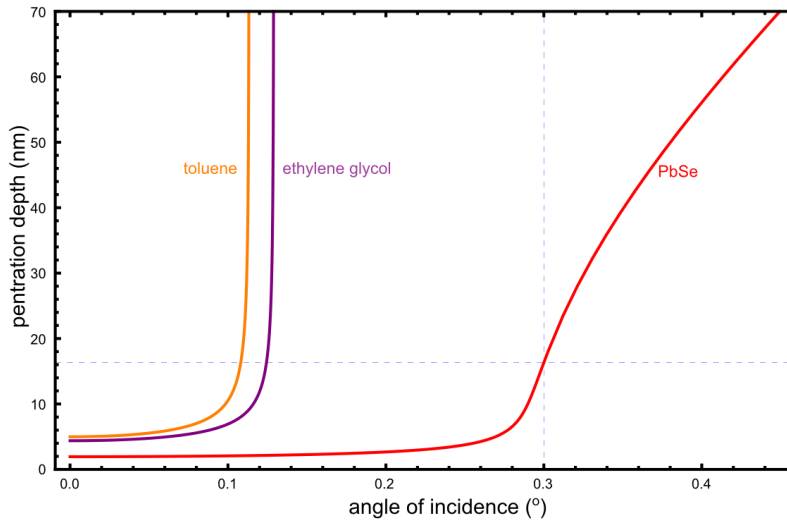
Figure S12: Calculation of the X-ray penetration depth as a function of incident angle. The red, purple and orange lines depict the penetration depths as function of incident angle for PbSe, ethylene glycol and toluene respectively. The blue dashed lines show the incident angle of the experiments (0.3°) and the corresponding penetration depth for PbSe (16.3 nm). Working at the critical angle of either toluene or ethylene glycol would result in a minute penetration of the X-ray photons into the PbSe superstructure.
