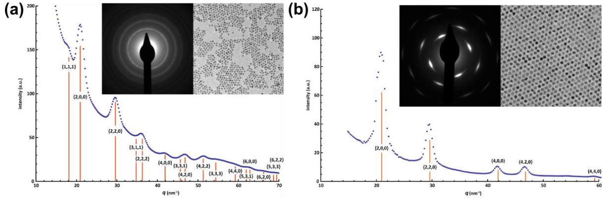
Figure S4: Azimuthally integrated electron diffraction patterns. The insets are the same images as (a) Fig. 1a and (b) Fig. 1g from the main text. Orange bars denote the positions of the atomic diffraction from PbSe (PDF card #00-006-0354). (a) All atomic reflections are visible, which indicates that the particles are not aligned with respect to the electron beam. (b) Only atomic reflections for nanocrystals with their \langle 100 \rangle direction perpendicular to the substrate are observed.
