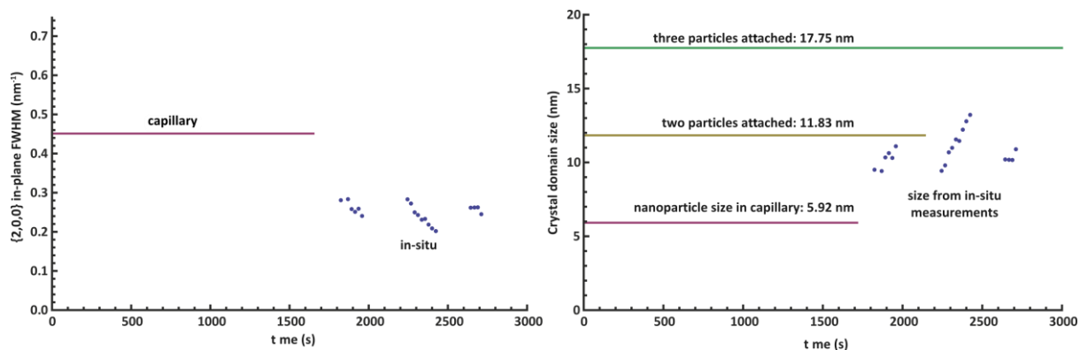
Fig S7: Evolution of the peakwidth of the horizontal {200} atomic reflection over time. Due to the large amount of experimental data, bad fits of the intensity profile were rejected from further analysis. (a) FWHM of the in-plane atomic {200} reflection over time. The purple line indicates the FWHM of the {200} diffraction of NCs dispersed in toluene, measured in a capillary. (b) The crystalline size is calculated as 2\pi/\Delta q , which corresponds to the Scherrer equation with K=1 if you realize that \Delta q = 4\pi/\lambda \cos(\theta) \Delta(2\theta)/2 .
