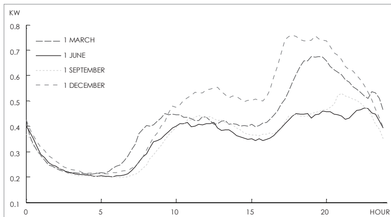
FIG.1.6 AVERAGE DEMAND PROFILE OF (400 RESIDENCES) WITH AN ANNUAL DEMAND OF 3400 KWH. (VELDMAN ET AL. 2013)
