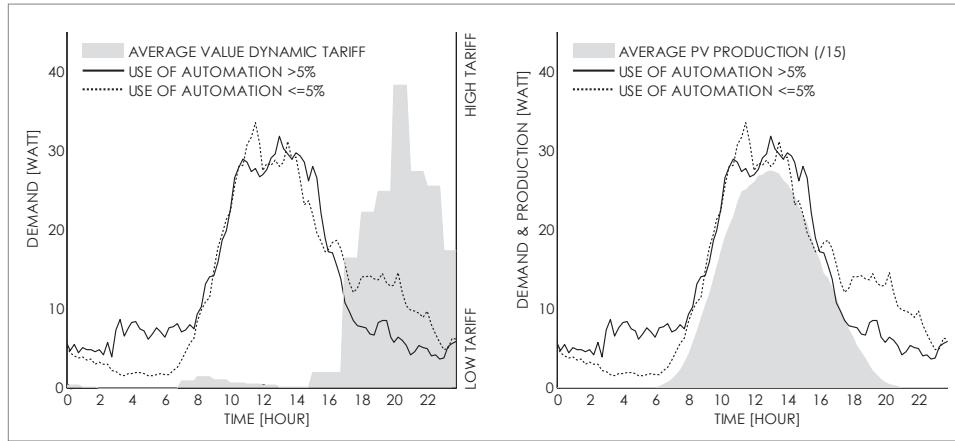
FIG. 5.4 ELECTRICITY DEMAND OF THE WASHING MACHINE FOR USERS OF AUTOMATION AND FOR NON-USERS WITH THE AVERAGE VALUE OF THE DYNAMIC TARIFF (LEFT) AND THE AVERAGE PV PRODUCTION (RIGHT)
