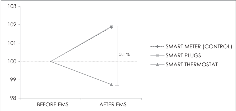
FIG. 2.1 MEAN NORMALIZED ELECTRICITY USAGE
