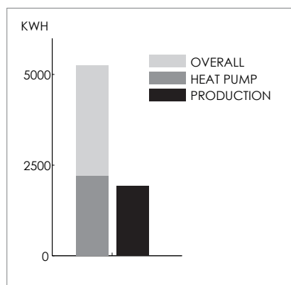
FIG.1.11 AVERAGE ELECTRICITY USE AND PRODUCTION IN MEULENSPIE, BREDA (05/13 - 05/14) (KLAASSEN ET AL. 2015)
