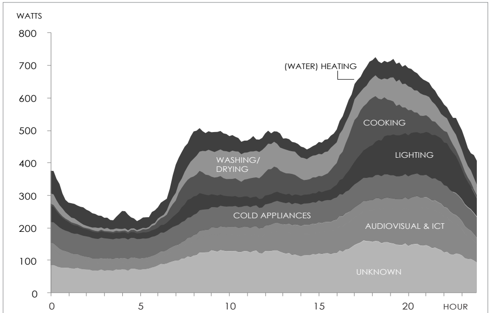
FIG.1.7 DEMAND PROFILE PER APPLIANCE GROUP OF UK HOUSEHOLDS (PALMER AND COOPER 2013)
