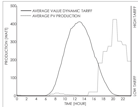
FIG.5.1 AVERAGE VALUE OF THE DYNAMIC TARIFF AND AVERAGE PV PRODUCTION DURING THE STUDY FROM 1 MARCH 2013 TO 1 MARCH 2014.
