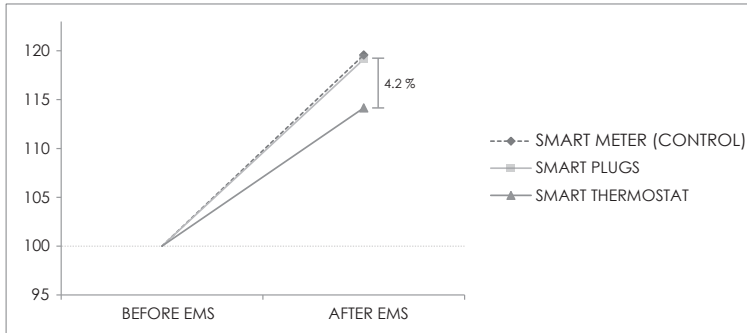
FIG.2.2 MEAN NORMALIZED GAS USAGE
