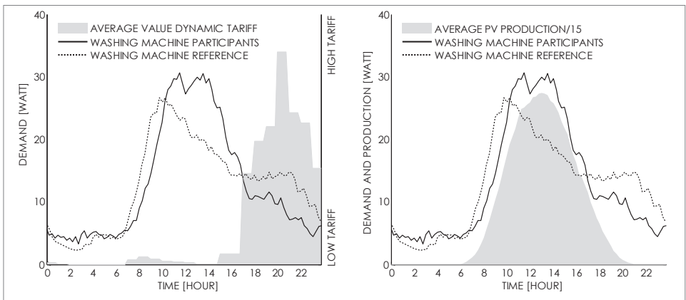
FIG.5.2 ELECTRICITY DEMAND OF THE WASHING MACHINE FOR PARTICIPATING HOUSEHOLDS AND THE REFERENCE GROUP WITH THE AVERAGE VALUE OF THE DYNAMIC TARIFF (LEFT) AND THE AVERAGE PV PRODUCTION (RIGHT)
