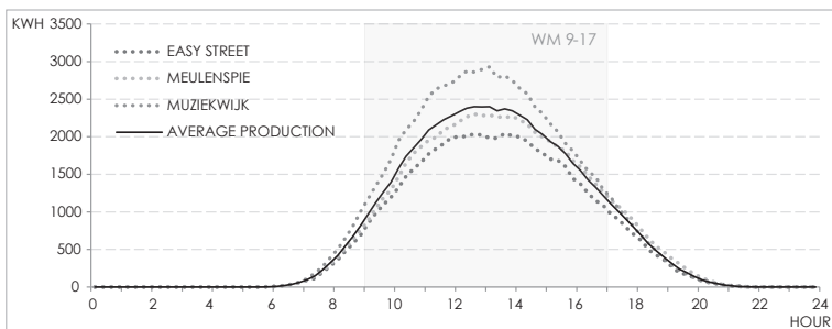
FIG. 6.3 TOTAL SOLAR PRODUCTION IN KWH PER AREA FROM 1-10-2013 TILL 1-10-2014
