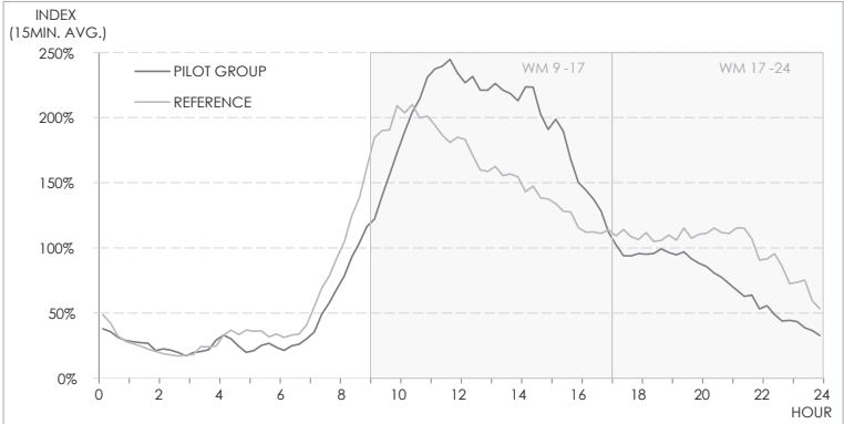
FIG. 6.5 AVERAGE LOAD PROFILES OF THE WASHING MACHINE FOR THE PILOT GROUP VS. THE REFERENCE GROUP
