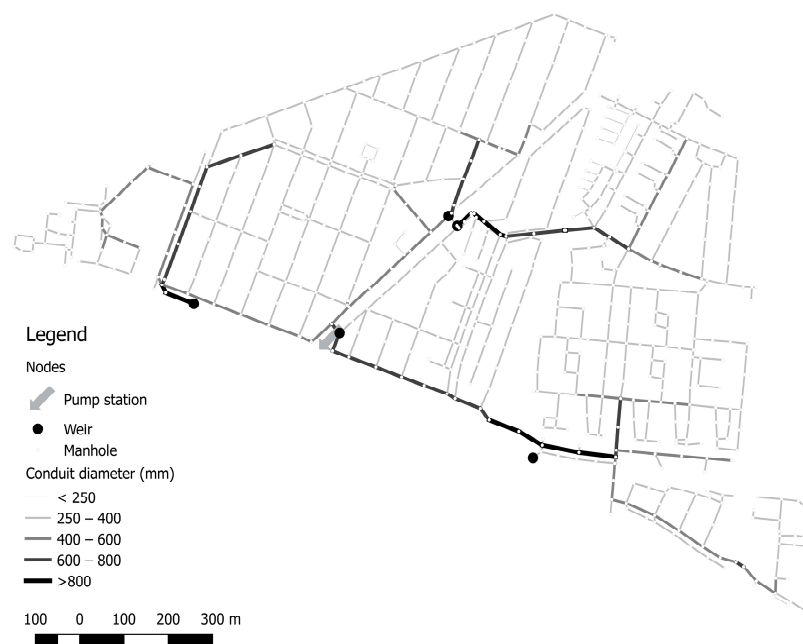
Figure 2. Layout catchment Tuindorp.
