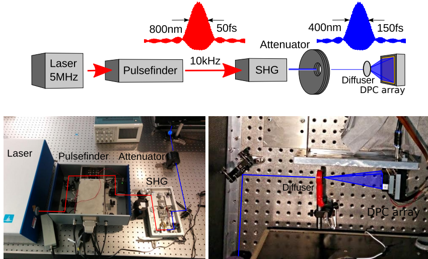
Figure 2. Schematic drawing and pictures of the experimental setup. The laser beam is led through a pulse-finder to adjust the rate to 10 kHz before its wavelength is halved by second harmonic generation (SHG). An attenuator wheel equipped with neutral density filters was used to adjust the laser intensity and a diffuser distributed the beam over the whole area of the DPC array.
