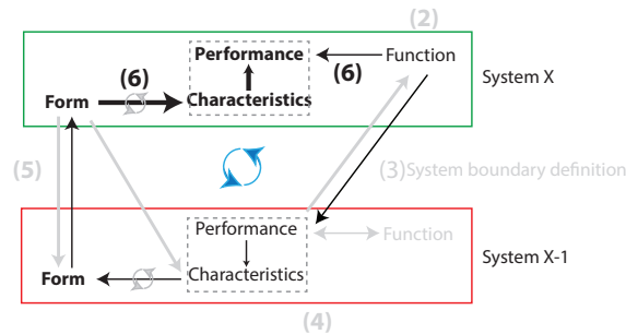
Figure 6-30. Step 6, defining performance of system X
