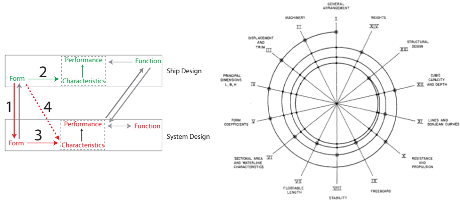
Figure 6-19. The model of cohesion and the design spiral (Evans, 1959)
