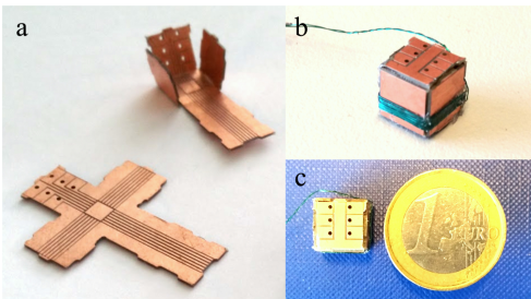
Fig. 4. a) Receiver cross-shape PCB. b) PCB housing the stimulation electronics folded into a box of 1 \text{ cm}^3 . The receiver coil is wrapped around the box. c) The receiver module size as compared to a one Euro coin.
