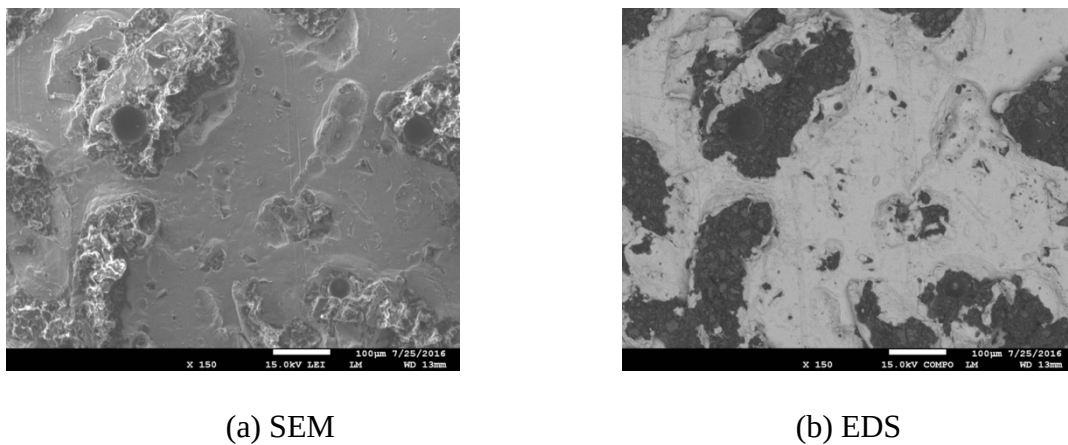
Figure 6. Typical SEM cohesive failure fracture surface (a) and corresponding EDS grey scale image (b).
