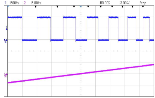
Fig. 18. Example of a measured output signal of the proposed system for a ramp input signal ( A_{1A}=14 dB).
