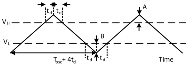
Fig. 6. The level detector delay as the major cause of non-linearity.
