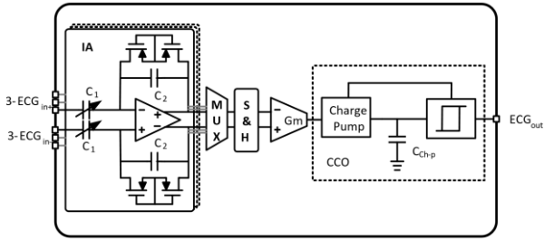
Fig. 2. Bio-potential measurement system architecture.
