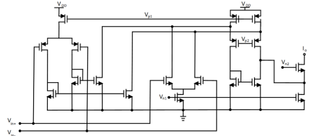
Fig. 9. Transconductor architecture: a rail-to-rail input folded cascode.
