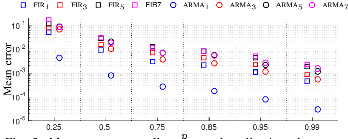
Fig. 3: Mean error over all nodes and realizations between sparsified and deterministic output for different values of p when \mathbf{L} = \mathbf{L}_n - \mathbf{I} .
