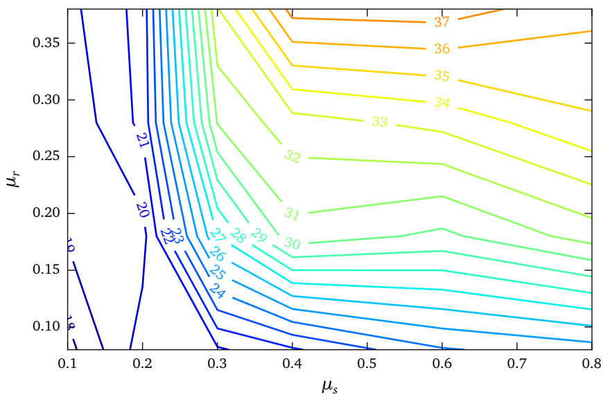
Figure 4.7: Effect of friction coefficients \mu_s and \mu_r on the angle of the free cone method.
