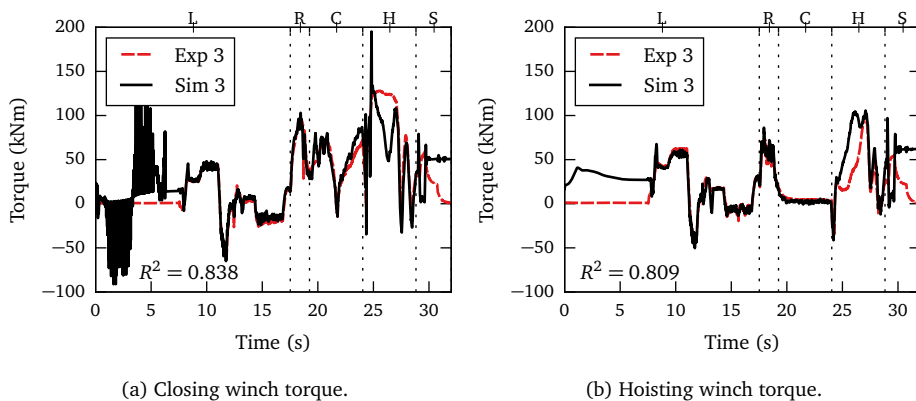
Figure 7.12: Closing and hoisting torque during simulation 3 and experiment 3 with a flat surface. Grab operation consists of lowering of the grab (L), resting on the surface (R), closing (C), hoisting (H) and being suspended from the crane (S).
