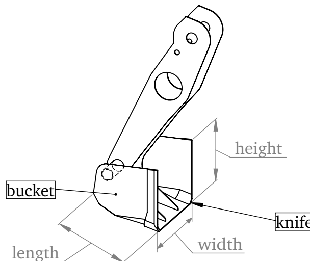
Figure 2.7: Grab parameters.
