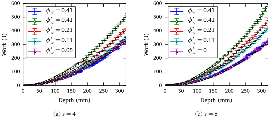
Figure 5.13: Penetration resistance with adjusted tip friction coefficient.
