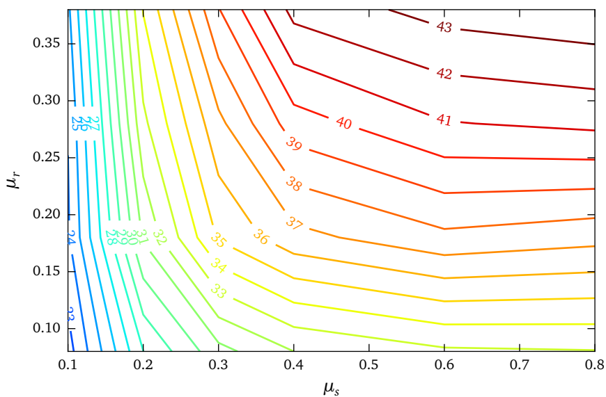
Figure 4.6: Effect of friction coefficients \mu_s and \mu_r on the angle of the ledge method.
