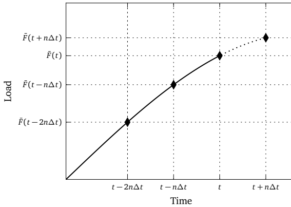
Figure 6.3: Force extrapolation required for MBD solver.
