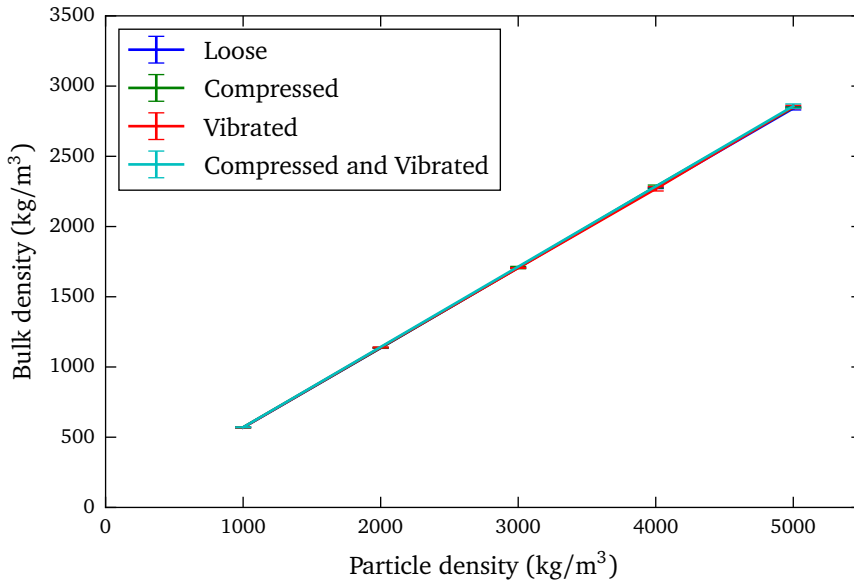
Figure 4.4: Bulk density.
