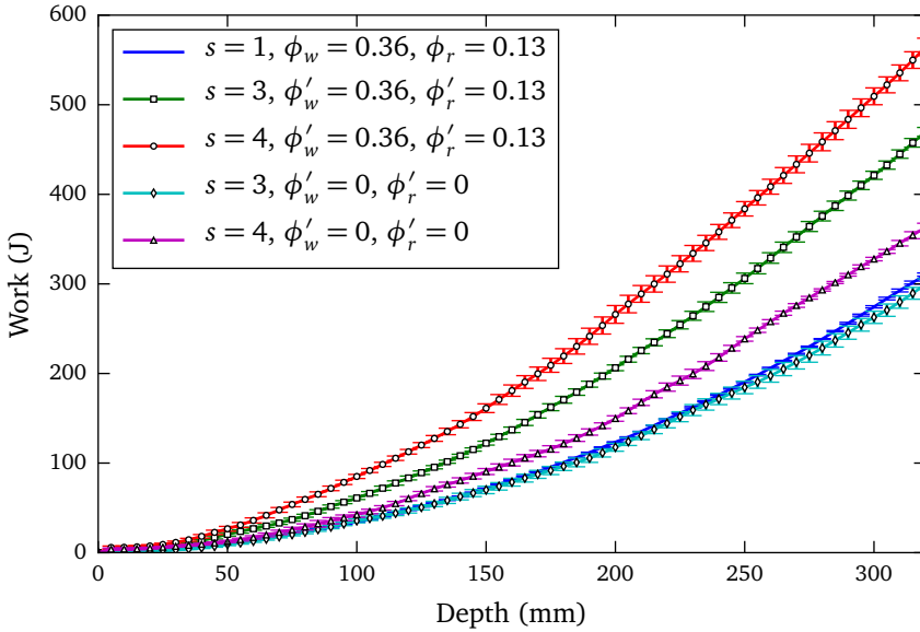
Figure 5.14: Penetration resistance for coarse grain rolling material model.
