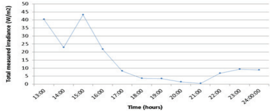
FIGURE C1.9: TOTAL MEASURED IRRADIANCE ( W/m^2 ) ON 31.05.2012 AT A NORTH ORIENTED OFFICE, SENSOR'S POSITION N2, TU DELFT.
