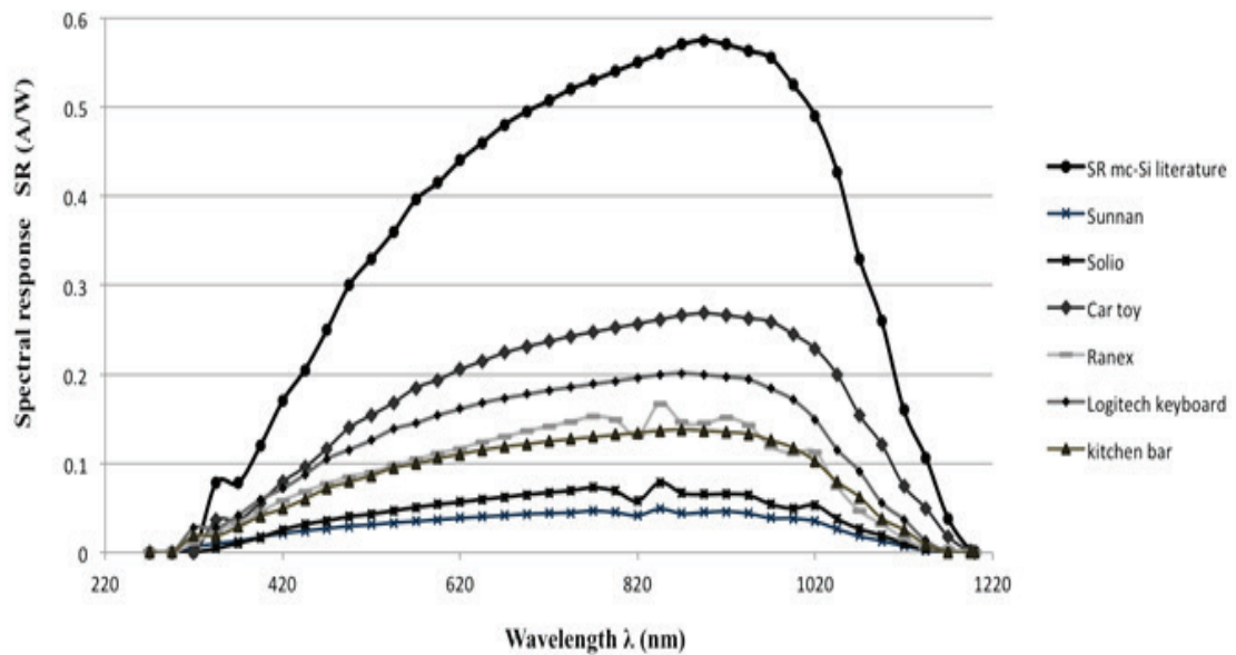
FIGURE 5.8: SPECTRAL RESPONSE OF mc-Si CELLS AS REPORTED IN LITERATURE (REICH ET AL., 2005), AND MEASURED FOR THE TESTED PV PRODUCTS (APOSTOLOU ET AL., 2014A, 2014B) UNDER STC.
