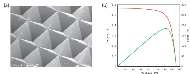
Fig. 7. a) SEM image of anti-reflective texture foil showing the inverted pyramid texture. b) IV-curve, measured independently by AIST in Japan, of the triple junction thin-film silicon PV module with an area of 1.42 \text{ m} \times 1.10 \text{ m} with anti-reflective texture foil.
