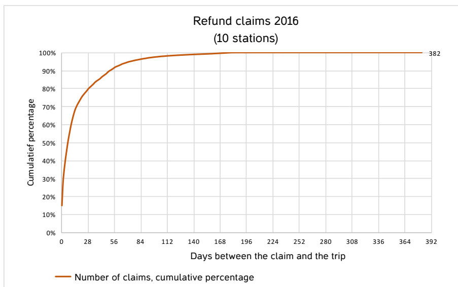
Figure 24: Claims from the ten stations in this study in 2016: after eight weeks, 92% of all claims from a given travel date had been received in the processing system.
