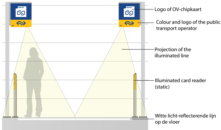
Figure 28: Schematic presentation of the revised proposal: separate signs and a projected illuminated line.
