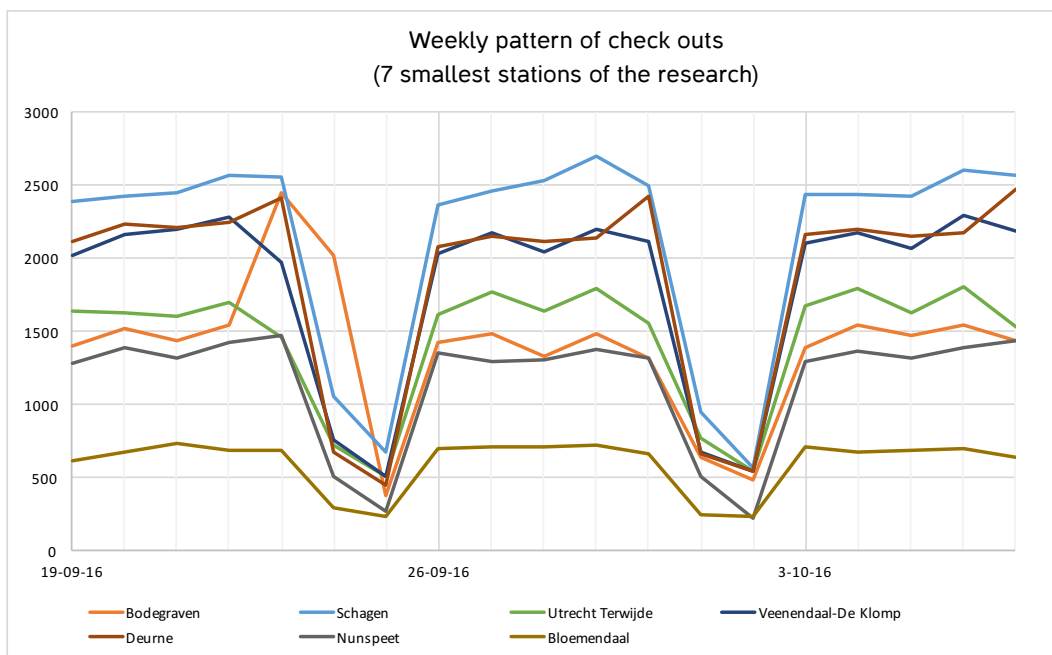
Figure 18: Number of check-outs per day for the seven smallest stations in this study.
