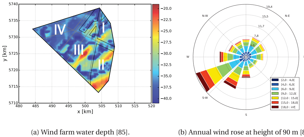
Figure 5.12: Description of the Borssele wind farm area, existing pipeline and telecom cables and water depth [85]. The color bar of the left figure represents the water depth in meters and the legend of the right figure presents the wind bins in m/s.
