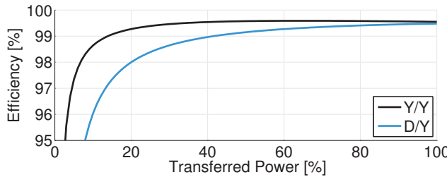
(a) Efficiency curves.
