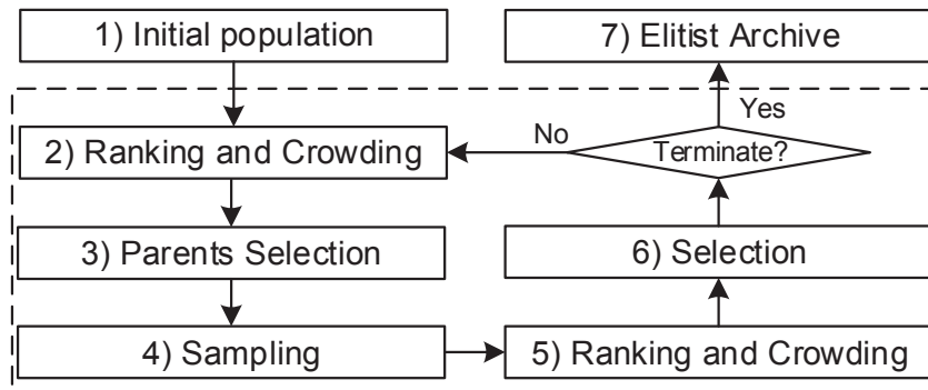
Figure 3.10: Flowchart of the NSGA-II.
