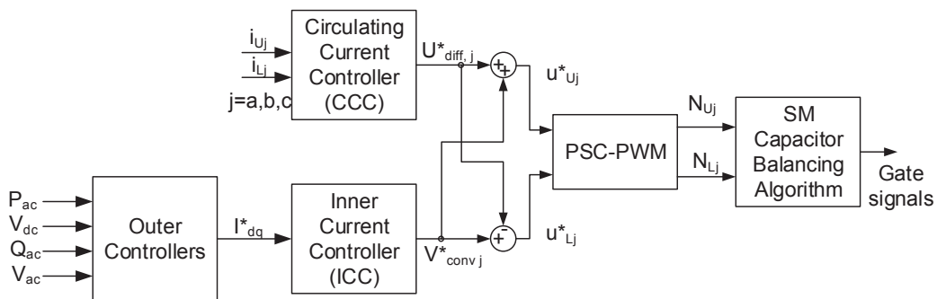
Figure 4.20: Control structure of the MMC station.
