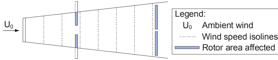
Figure 3.5: Wake growth and wind speed decrease according to the Katic-Jensen model.
