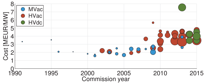
Figure 1.5: Cost per MW installed of the European OWFs composed of five or more turbines [9, 10]. Monetary values updated considering a Eurozone inflation of 1.85% [19].
