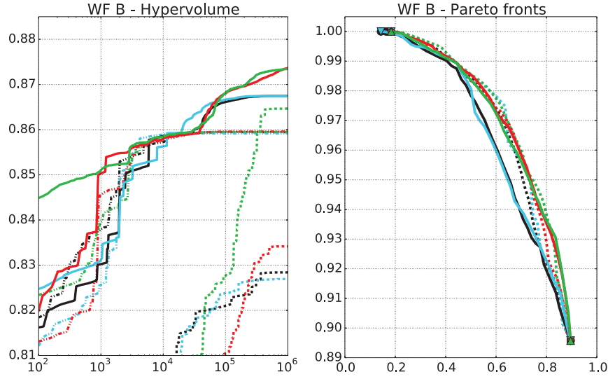
Figure 3.17: The left plot shows the average hypervolume obtained with the different algorithms with 8 RD (dash-dotted), 4 RD (dotted) and with the multi-step (solid) approach for wind farm area B. The x-axis shows the number of fitness valuations and the y-axis displays the hypervolume. The right plot shows the aggregated Pareto fronts between all the different step sizes (dotted) and the aggregated Pareto fronts obtained with the multi-resolution scheme (solid). The x- and y-axes show the optimization goals, respectively. For both plots: MOGOMEA - red; o-MOGOMEA - green; NSGA-II - black; c-NSGA-II - blue.
