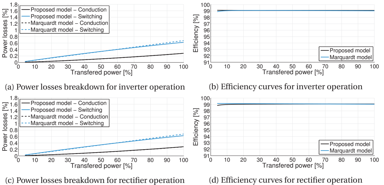
Figure 4.17: Marquardt and proposed model with Marquardt's assumptions.
