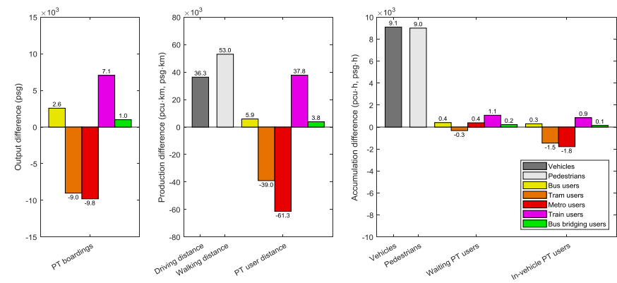
Figure 6.13. Differences of the emergency scenario compared to a normal day in the model without subcritical delays.
