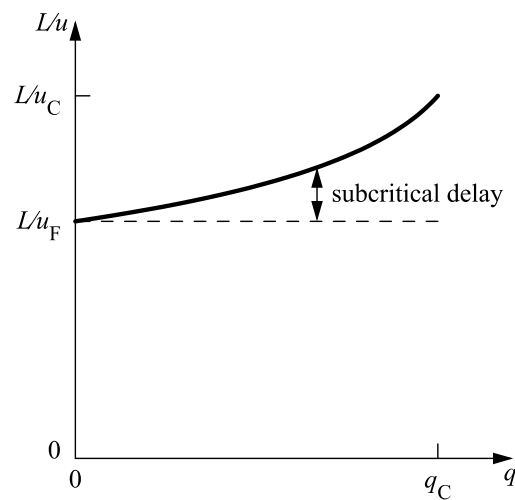
Figure 5.1. Link travel time L/u in stationary homogenous free-flow conditions as a function of flow q .
