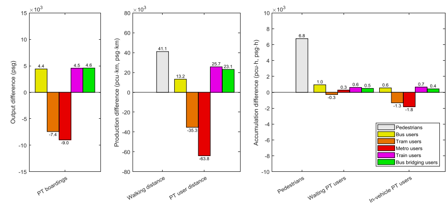
Figure 6.16. Differences of the emergency scenario compared to a normal day in the model without car traffic.
