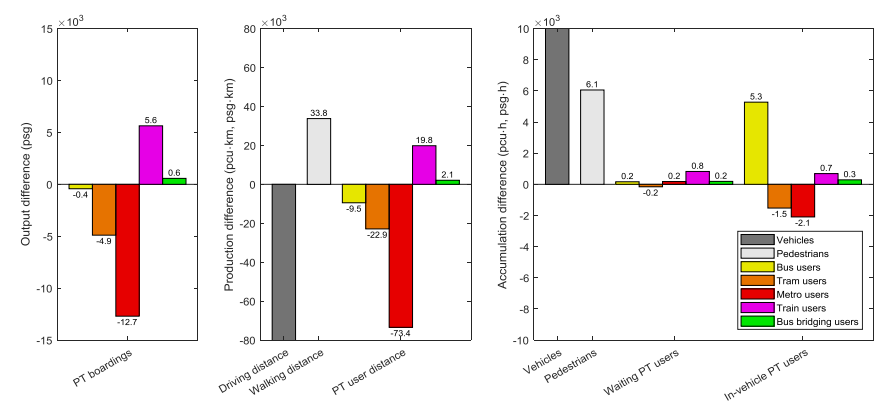
Figure 6.15. Differences of the emergency scenario compared to a normal day in the model without en-route choice for cars.
