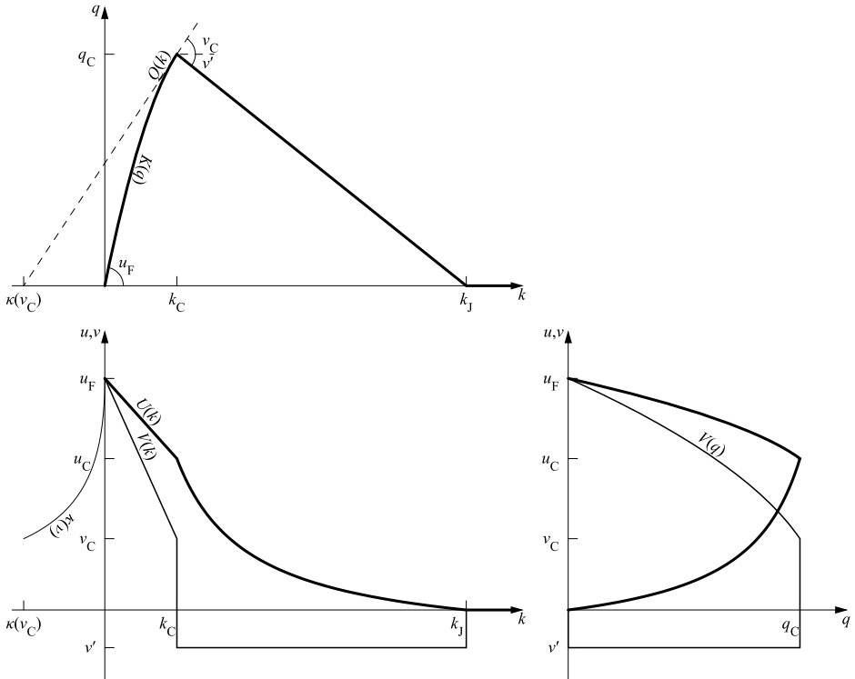
Figure 5.5. Smulders fundamental diagram (thick solid lines) and corresponding wave speeds (medium solid lines), including the extension beyond jam density.
