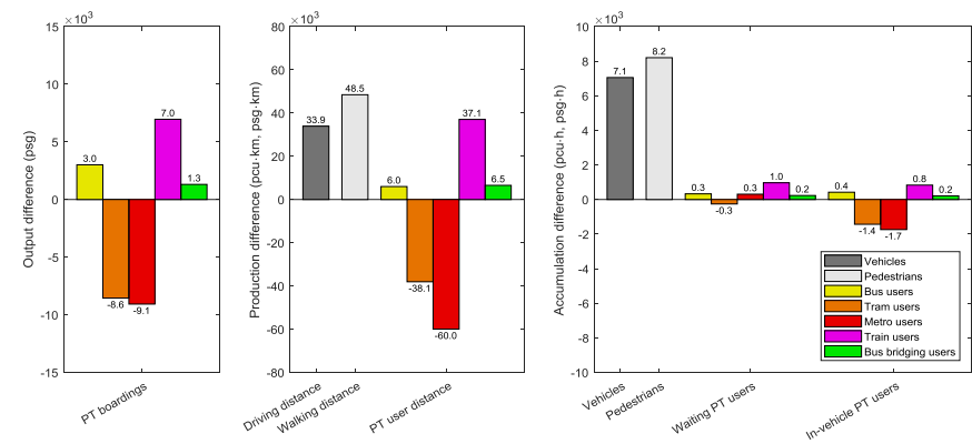
Figure 6.14. Differences of the emergency scenario compared to a normal day in the model without traffic lights.
