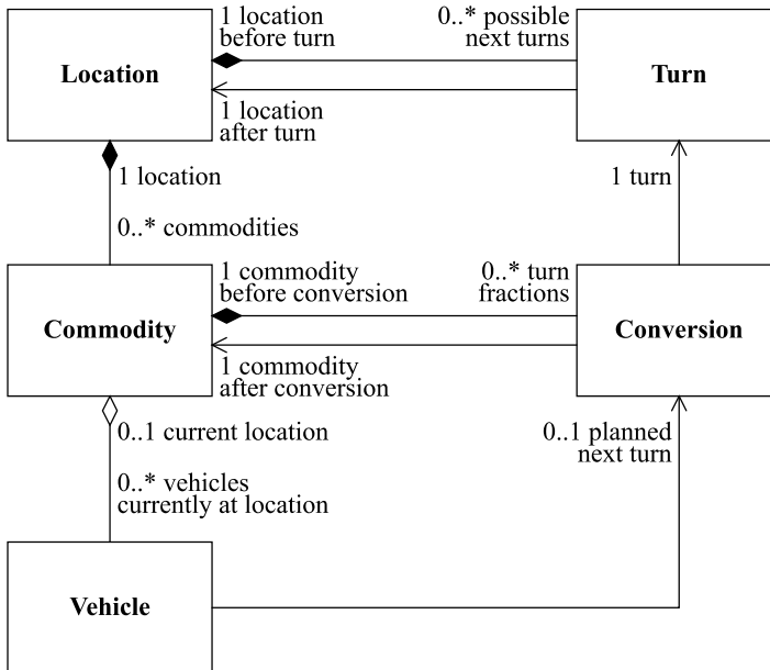
Figure 2.3. Unified Modelling Language class diagram of commodities.
