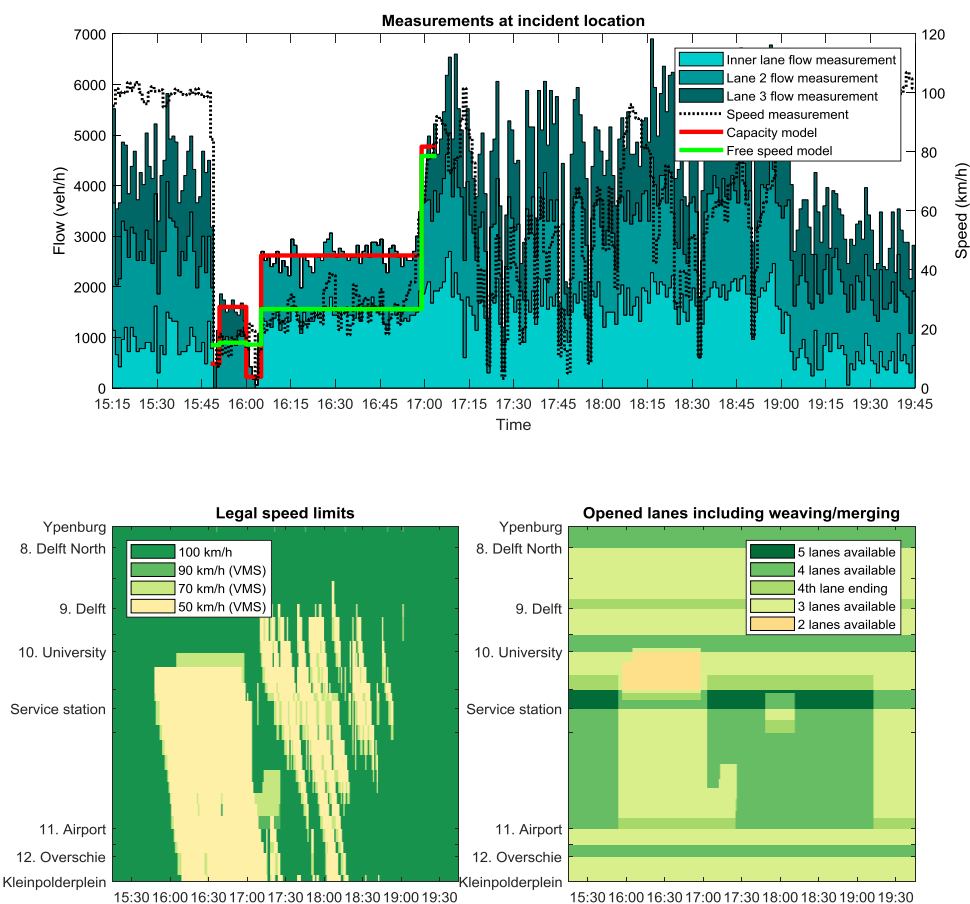
Figure 5.10. A13 flow at crash location and applied traffic control.
