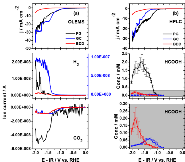
Figure 2. (a) Online electrochemical mass spectrometry and (b) online HPLC during CO 2 reduction on immobilized InPP on different substrates in 0.1 M phosphate buffer of pH 9.6.
