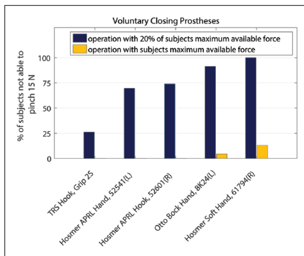
Figure 4. Pinching 15 N repetitively with five voluntary closing prostheses fatigue free is impossible for 26%–100% of prosthesis users. Fatigue-free operation is considered at 20% of users' maximum cable force 5 and is desired for ADL. Cable forces required to pinch 15 N with five voluntary closing prostheses vary between 33 and 131 N. 2 The maximum strength of 13% of prosthesis users is insufficient to pinch 15 N with the Hosmer Soft Hand.
