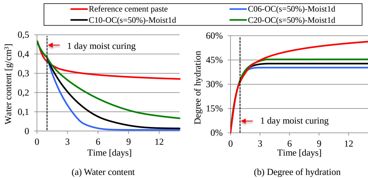
Fig. 5.6 Calculated water content and calculated average degree of hydration of the coatings ( w/c = 0.3 ) with different thicknesses (6, 10 and 20 mm). The coatings are applied on substrate OC ( s = 50\% ). One day moist curing is applied, followed by exposure to 50% RH until 14 days. The reference cement paste ( w/c = 0.3 , no substrate) is cured under sealed condition.
