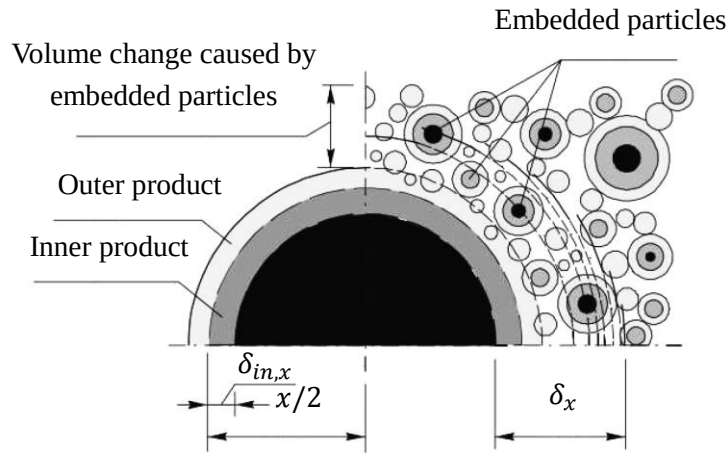
Fig. 4.16 Basic principles of HYMOSTRUC3D and formation of hydration products (by van Breugel [8]).
