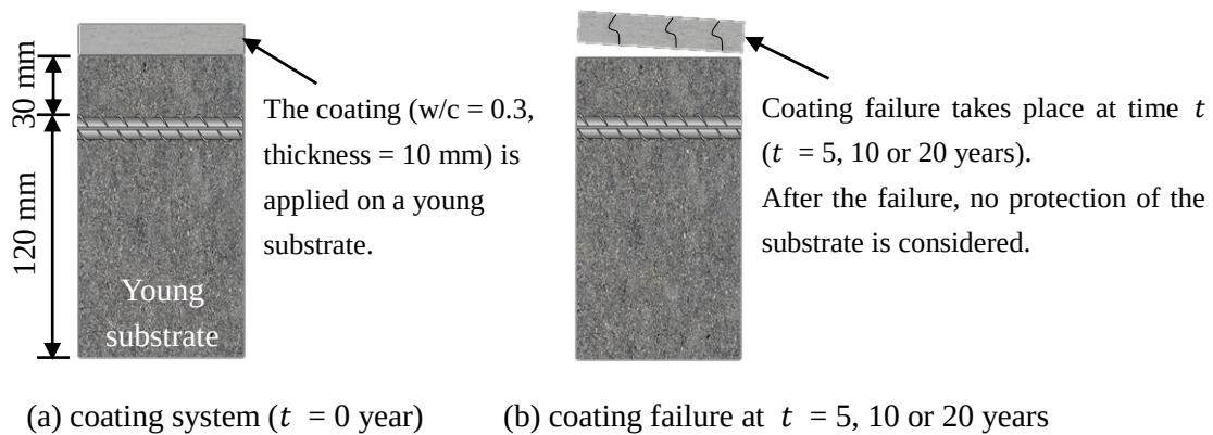
Fig. 6.13 Coating failure in the coating system. Coatings are applied on young substrates. After t (5, 10 or 20) years, the coating fails due to cracking or de-bonding.
