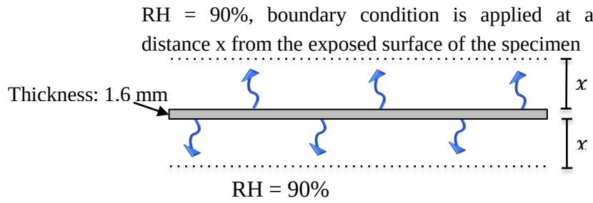
Fig. B.3 Schematic illustration of a cement paste ( w/c = 0.3 ) hydrating under RH = 90\% . The boundary condition is applied at a distance x ( x = 30, 60 or 100\text{ mm} ) from the surfaces of the specimen.
