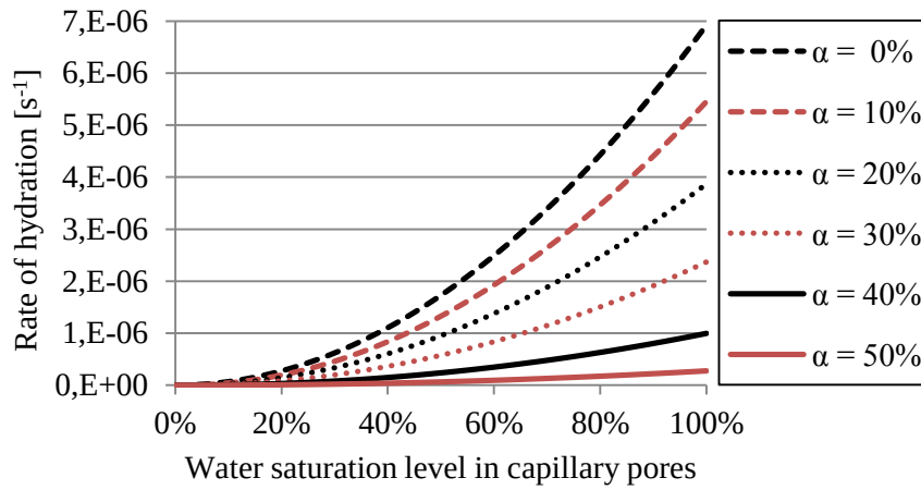
Fig. 4.20 Influence of water saturation level in capillary pores on the rate of hydration \alpha of the cement particles in a cement paste with w/c = 0.3 .
