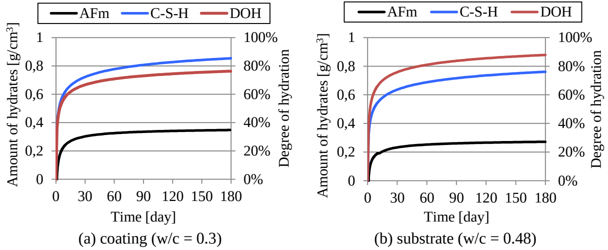
Fig. 6.8 Evolution of degree of hydration and the amounts of hydrates ([g per cm³ of cement paste]). (a) coating (w/c = 0.3), (b) substrate (w/c = 0.48). The coating and the substrate are cured under saturated condition.
