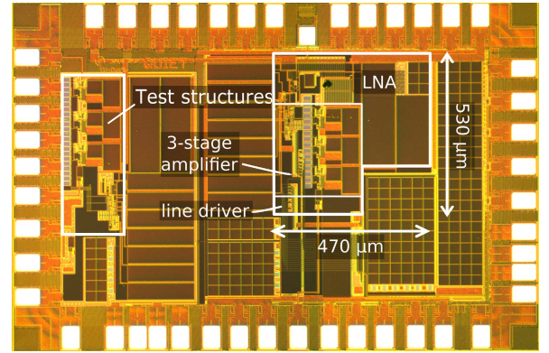
Fig. 12. Chip micrograph of the noise-canceling LNA plus three-stage diode-loaded amplifier and 50- \Omega driver.
