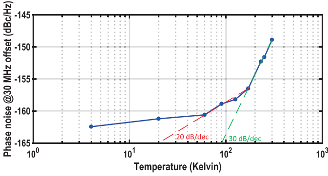
Fig. 23. PN at 30 MHz offset from a 6.3 GHz carrier versus temperature.
