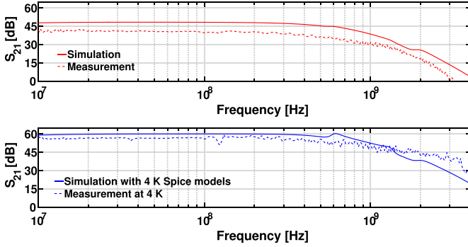
Fig. 14. Comparison of S_{21} between measurements and simulations both at 300 K and 4 K with the use of the developed SPICE models for low temperatures.
