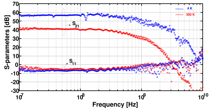
Fig. 13. Measured S-parameters of the LNA at room temperature and at 4 K.
