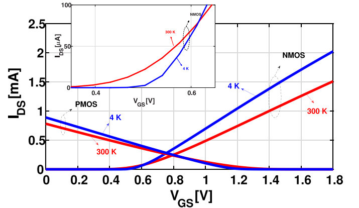
Fig. 5. I_D - V_G characteristic of thin-oxide NMOS and PMOS in 160-nm CMOS technology. Inset: clear shift in threshold voltage for the NMOS characteristics.
