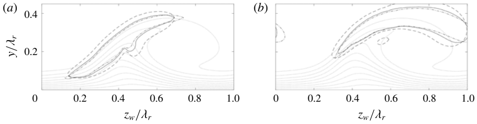
FIGURE 33. |\tilde{u}_w|/\max|\tilde{u}_w| = 1/6 for Reynolds number: 10^{-0.8}Re (dashed line), nominal (solid) and 10^{0.8}Re (dash-dotted) for type I (a) and II (b). \overline{U}_w/\overline{U}_e levels 0.1, 0.2, ..., 0.9 (dotted).
