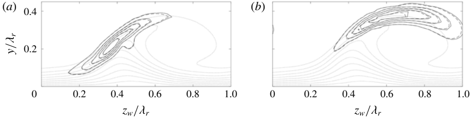
FIGURE 21. Temporal (solid lines, \alpha \in \mathbb{R} ) and spatial (dashed lines, \omega \in \mathbb{R} ) eigenfunctions ( |\tilde{u}_w| / \max |\tilde{u}_w| levels span [1/6, 5/6] with \Delta = 1/6 ) for type I (a, \omega_r \lambda_r / \bar{U}_e = 4.5967 ) and II (b, \omega_r \lambda_r / \bar{U}_e = 7.354 ). \bar{U}_w / \bar{U}_e levels 0.1, 0.2, \dots , 0.9 (dotted).
