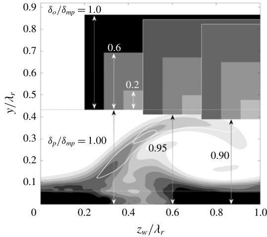
FIGURE 18. Overlap region definition and variations. In-plane \overline{U}_w -shear magnitude of the strong vortex for N_{fr} = 500 (8 filled contours from 0 to 7 in \overline{U}_e/\lambda_r -units). |\tilde{u}_w|/\max|\tilde{u}_w| = 0.5 for most unstable type I and II modes (white contours). Near-wall region ( y/\lambda_r \leq 0.061 ) and upper limit PIV domain ( y/\lambda_r = 0.433 ) (dotted lines).
