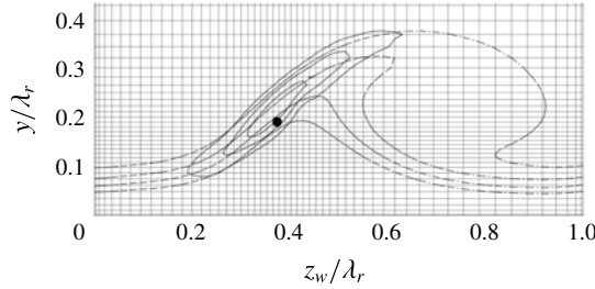
FIGURE 6. Zoom of mapped Chebyshev grid ( 55 \times 55 nodes). |\tilde{u}_w|/\max |\tilde{u}_w| of type I (solid contours at 25 %, 50 % and 75 %). \bar{U}_w/\bar{U}_e levels 0.6, 0.7, 0.8 and 0.9 (dash-dotted). Position of (\bar{V}, \bar{W}_w) -field saddle point (solid circle).
