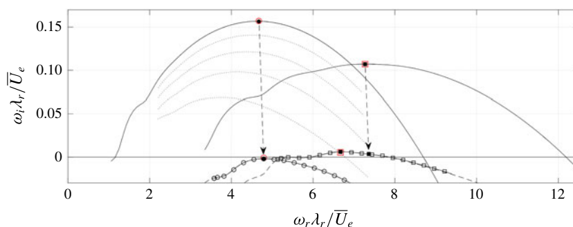
FIGURE 27. (Colour online) Type I (circles) and II (squares) temporal stability branches for the weak vortex using N_z \times N_y = 55 \times 55 (dashed lines) and 90 \times 90 (solid) grid nodes. Strong vortex branches (solid without open symbols). Arrows link type I and II modes with \alpha \lambda_r = 6.2 and 8.6 (filled symbols), respectively, on the different vortices. All most unstable eigenvalue symbols are filled. Eigenvalues corresponding to domain containing both strong and weak primary vortices using N_z \times N_y = 140 \times 70 (red symbols). Branches corresponding to the interpolated base flows with \chi = 0.2, 0.4, 0.6 and 0.8 (dotted lines, bottom to top).
