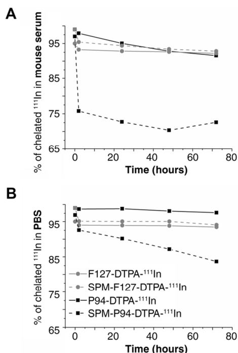
Figure 3. In vitro stability of ^{111}\text{In} radiolabeled Pluronic nanocarriers at 37°C after dilution in (A) mouse serum and in (B) PBS for 72h.
