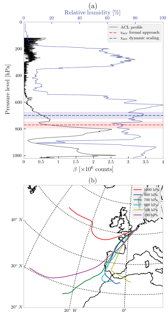
Figure 8. (a) Radiosonde profile of relative humidity (blue), plotted alongside an averaged raw attenuated backscatter profile (black) from the ceilometer at De Bilt, the Netherlands. Both profiles are approximately around 13:00 UTC. The red and blue dashed lines represent retrieved aerosol layer height using the formal approach and the dynamic scaling method, respectively. The red- and blue-shaded boxes represent the aerosol layer from the respective retrieval methods. (b) Back trajectories calculated for 17 October 2017 at 13:00 UTC with the end point at De Bilt, and the sources going back to 3 days.
