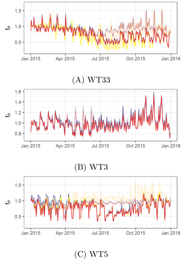
Figure 6: Performance factor for selected underperforming turbines based on MOB (blue), RF (yellow, not used in farm B due to missing data) and GP model (red). Farm average performance in transparent colours.
