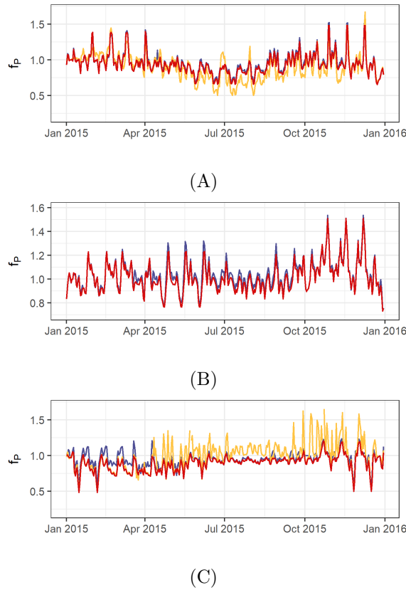
Figure 5: Mean performance ratio of each farm based on MOB (blue), RF (yellow) and GP model (red).
