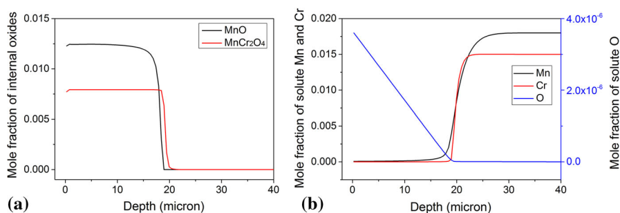
Fig. 3 Simulated concentration profiles of a internal oxides and b solute Mn, Cr and O after annealing the Fe–1.9Mn–1.6Cr steel at 950 °C for 16 h in Ar + 5 vol% H 2 gas mixture with a dew point of 10 °C
