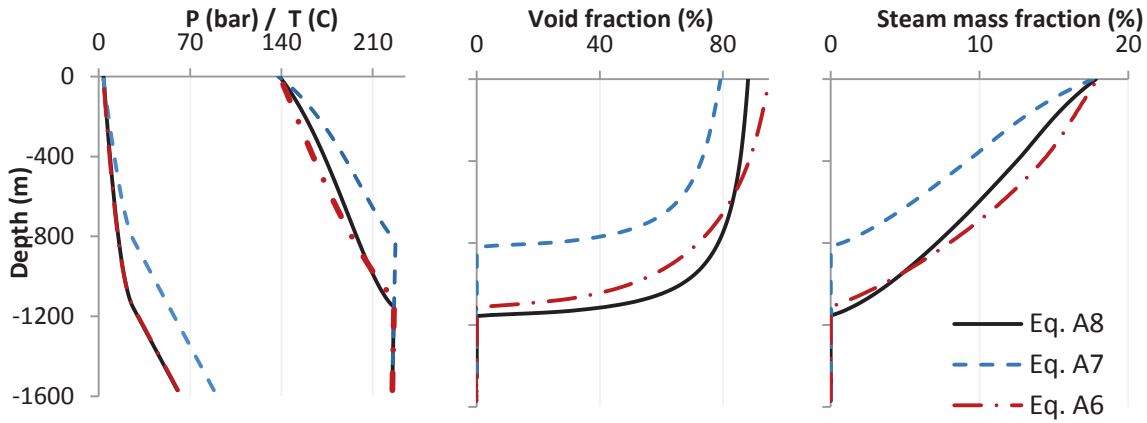
Figure 10: Effect of different constitutive models for the drift flux profile parameter, at t = 60 hour
