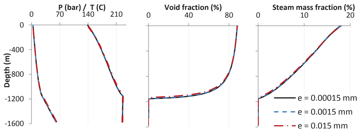
Figure 9: Effect of wellbore roughness, at t = 60 hour
