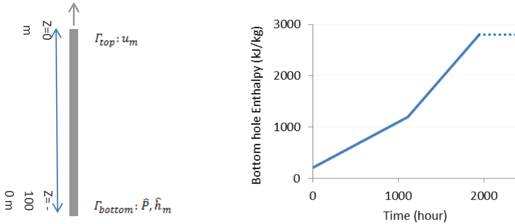
Figure 2: Geometry and the boundary conditions
