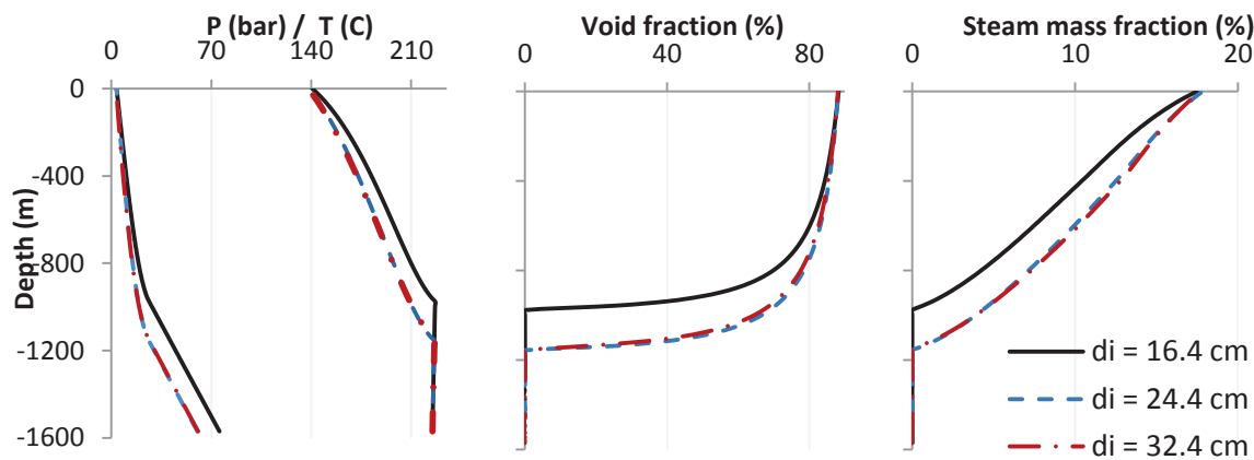
Figure 8: Effect of well diameter, at t = 60 hour
