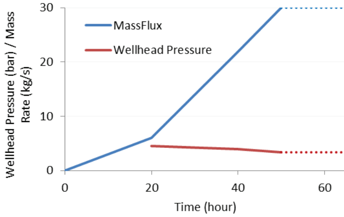
369 370 Figure 5: Wellhead pressure and mass flow rate boundary conditions
