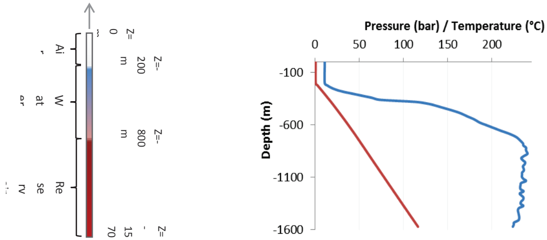
Figure 4: Down hole measured stable temperature (Blue log) and pressure (red log) along the NWS-1 wellbore; The top 200 meter of well has been filled with air in the natural state.
