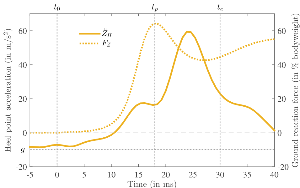
Fig 7. A typical example of the vertical heel point acceleration \ddot{Z}_H in the same figure as vertical ground reaction force F_Z as reference (same measurement as in Figs 3 and 4). As in Fig 4 the start of impact is shown by a vertical dotted line indicated by t_0 , the instant of the vertical force peak is indicated by t_p and the end of heel strike, which is defined as zero vertical heel velocity, by t_e . Here also the gravitational acceleration g is shown.
