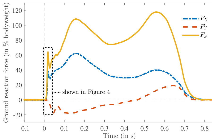
Fig 3. A typical example of the measured ground reaction force acting on the right foot defined in the global coordinate system XYZ as a percentage of body weight (727 N) as a function of time, where the subscript X corresponds to mediolateral, Y to anterior-posterior and Z to vertical component of the force. A dotted rectangle is shown to indicate the initial part of the stance phase where heel strike takes place. The ground reaction forces of this initial part is shown in Fig 4.
