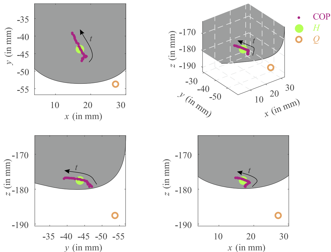
Fig 5. A typical example of the location in the local xyz coordinate system of the center of pressure (COP) points during the impact phase used to define the heel point H . The COP point at each instant is transformed to the local xyz coordinate system (see Fig 1), where the mean of these points are used to define the heel point H . The progression of the COP points as a function of time is indicated by the arrow. A point Q is defined in order to perform a parameter sensitivity analysis. This point lies 1 cm away from H in lateral ( x ), posterior ( -y ) and inferior ( -z ) direction. The gray areas are drawn to roughly indicate the boundaries of the undeformed heel.
