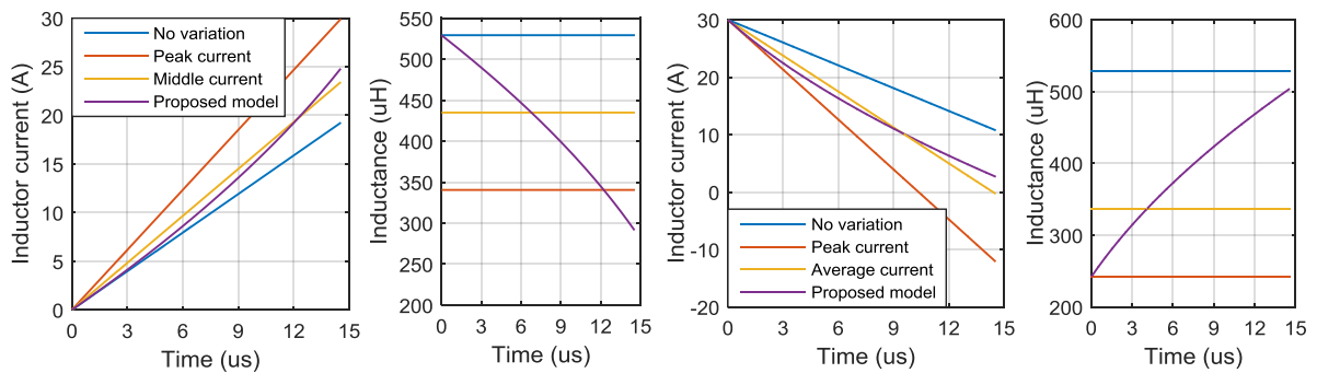
Fig. 4. Inductor current and inductance estimated by four methods for L_0 = 529.2 \mu H using 60\mu KoolMμ core with (left) V_L = 700V , \Delta t = 15 \mu s , i_{L(0)} = 0 and (right) V_L = -700V , \Delta t = 15 \mu s , i_{L(0)} = 30A ;
