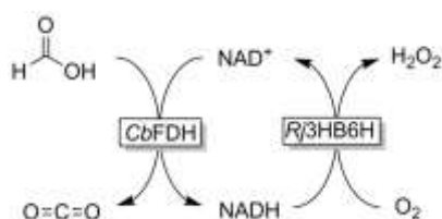
Scheme 3. The final oxidation step (formic acid to CO 2 ) producing H 2 O 2 using a combination of formate dehydrogenase (CbFDH) and 3-hydroxybenzoate-6-hydroxylase (Rj3HB6H).
