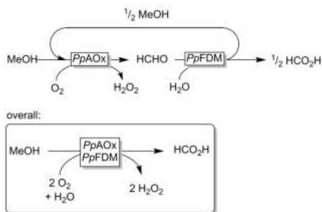
Scheme 2. The proposed bienzymatic cascade comprising alcohol oxidase (AOx) and formaldehyde dismutase (FDM) for the overall double oxidation of methanol to formic acid generating two equivalents of \text{H}_2\text{O}_2 .
