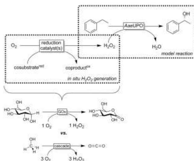
Scheme 1. Schematic representation of the new in situ H 2 O 2 generation system and the model reaction used in this study. The unspecific peroxygenase from Agrocye aegerita (AaeUPO) catalyses the chemo- and stereospecific conversion of ethyl benzene to enantiopure ( R )-1-phenylethanol (model reaction). In situ provision with H 2 O 2 is achieved by catalytic reduction of ambient oxygen (O 2 ) (regeneration reaction). Shown below are: (1) the established method using glucose oxidase (GOx)-catalysed single oxidation of glucose generating one equivalent of H 2 O 2 and (2) the envisioned 'through oxidation' of methanol to CO 2 generating 3 equivalent of H 2 O 2 .
