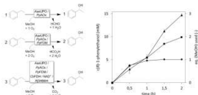
Figure 2. Comparison of the different cascades for methanol oxidation to promote the AaeUPO-catalysed hydroxylation of ethyl benzene. Diamonds (◆): using PpAOx only; Squares (■): PpAOx combined with PpFDM and Triangles (▲): the entire cascade. General conditions: [ethylbenzene] = 15 mM, [methanol] = 5 mM, [AaeUPO] = 50 nM, [PpAOx] = 60 nM in 100 mM phosphate buffer (pH 7.0), T = 30°C; ■: [PpFDM] = 590 nM; ▲: [PpFDM] = 590 nM, [NAD + ] = 1.6 mM, [2,5-dihydroxybenzoic acid] = 1 mM, [Rj3HB6H] = 11 μM, [CbFDH] = 1 μM.
