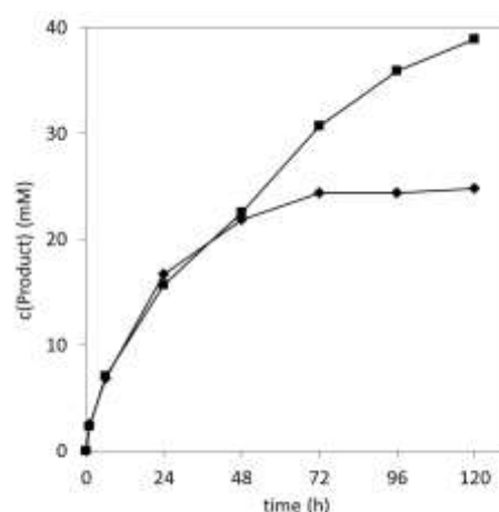
Figure 1. Enzymatic hydroxylation of ethylbenzene in the absence ( \blacklozenge ) and presence ( \blacksquare ) of PpFDM. Conditions: [ethyl benzene] = 50 mM, [methanol] = 200 mM, [AaeUPO] = 100 nM, [PpAOx] = 60 nM, [PpFDM] = 295 nM in 100 mM phosphate buffer (pH 7.0), T=30^\circ\text{C} . For the sake of clarity, both ( R )-1-phenyl ethanol and acetophenone are shown, please see the text for further information.
