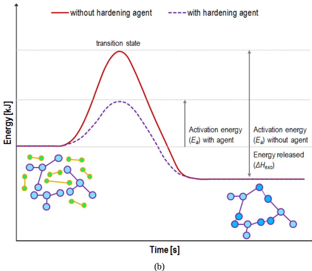
FIGURE 1 Crosslinking of epoxy modified bitumen: (a) stepwise polymerization of epoxy in the bituminous matrix; and (b) exothermic chemical reaction diagram
