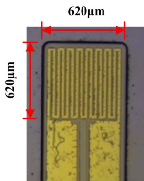
Fig. 3.3: Flexible micro-temperature sensor developed by Lee et al. [33].
