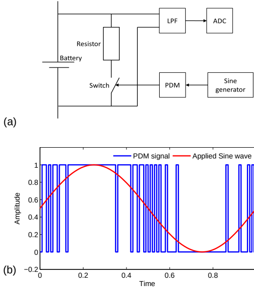
Fig. 5.2: Simplified measurement scheme of a printed-circuit-board assembled in parallel to a battery (a) and a schematic representation of a pulse-density-modulated (PDM) signal (blue line) of a sine wave (red line) (b).
