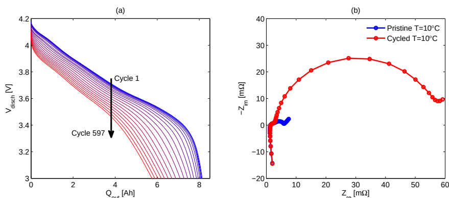
Fig. 4.9: Voltage discharge curves upon cycling an NCA battery (a), and impedance spectra of a pristine and cycled NCA battery at 60% SoC and 10°C.
