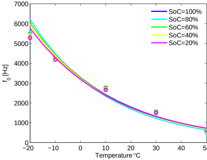
Fig. 4.8: Zero-intercept frequency as a function of temperature for a pristine LiFePO₄ battery.
