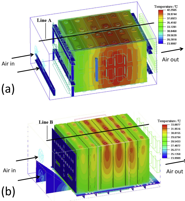
Fig. 2.4: Examples of thermal simulations of a Li-ion battery pack, containing 12 180 Ah batteries, at the end of 1C-rate discharging, using forced convection with one-directional air flow (a) and forced convection with two-directional air flow (b). Modified from Ref. [90].
