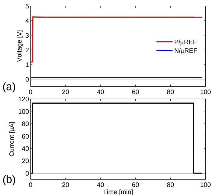
Fig. 8.3: Voltage between P (red line) and N with respect to \mu\text{REF} (blue line) (a), and deposition current (b) during metallic lithium deposition. Note that the depositions were performed sequentially.
