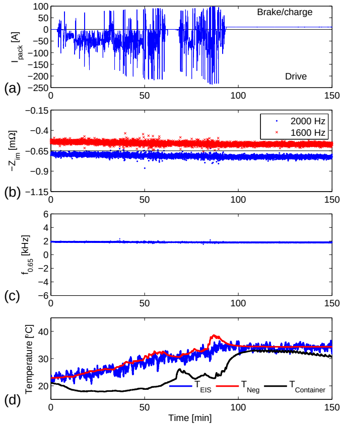
Fig. 5.14: Battery pack current (a), imaginary impedance at 1600 Hz (red symbols) and 2000 Hz (blue symbols) (b), interpolated NZIF f_{0.65} -values (c), and temperature (d) as a function of measurement time during an EV test drive.
