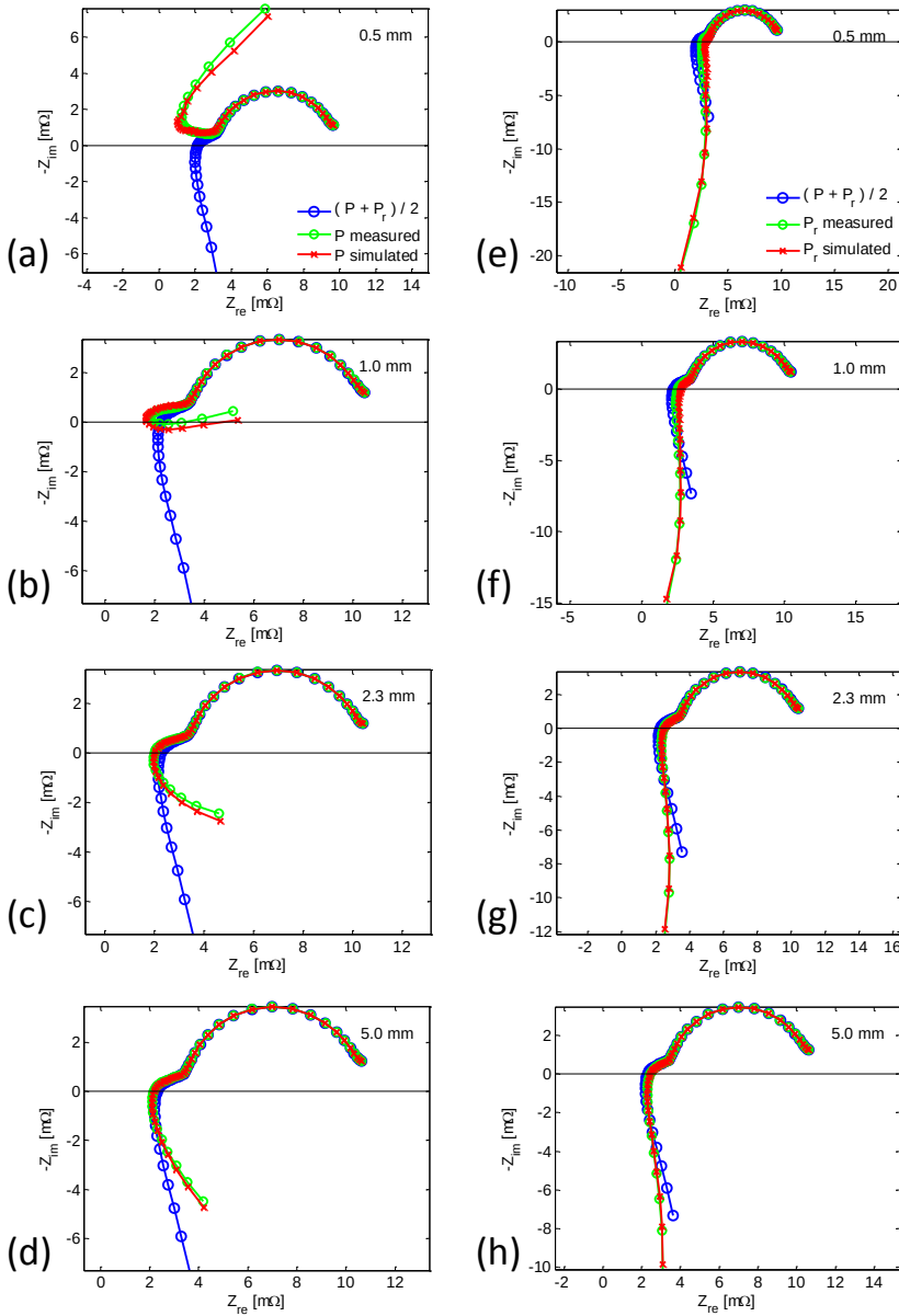
Fig. 7.9: Measured and simulated impedance spectra of P with respect to various \mu\text{REF} with indicated lengths (0.5, 1.0, 2.3 and 5.0 mm) obtained with standard (a-d) and reversed cable connection set-up (e-h). The blue curves show the compensated (averaged) measured impedance of P, the green curves show the measured (uncompensated) P impedance, including artefacts, and the red curves shows the uncompensated simulations.
