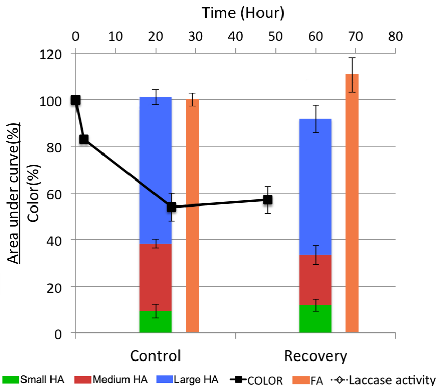
Fig 6. HA removal by deactivated immobilized fungi. SEC results of HA and FA are presented as area under the curve (lower X-axis). Color removal (%) was monitored during the incubation period (upper X axis). Results are presented as the average of triplicates \pm SD.
