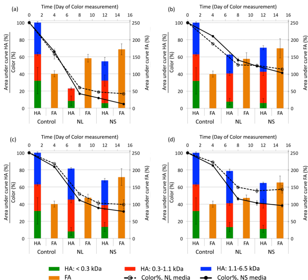
Fig 2. HA color removal during the fungal treatment and SEC results of the HA and FA content of the wastewater (area under the curve) before (uninoculated control) and after the fungal treatment (after recovery of sorped HA) in NL and NS media. a: T. versicolor , b: P. chrysosporium , c: P. pulmonarius and d: P. ostreatus
