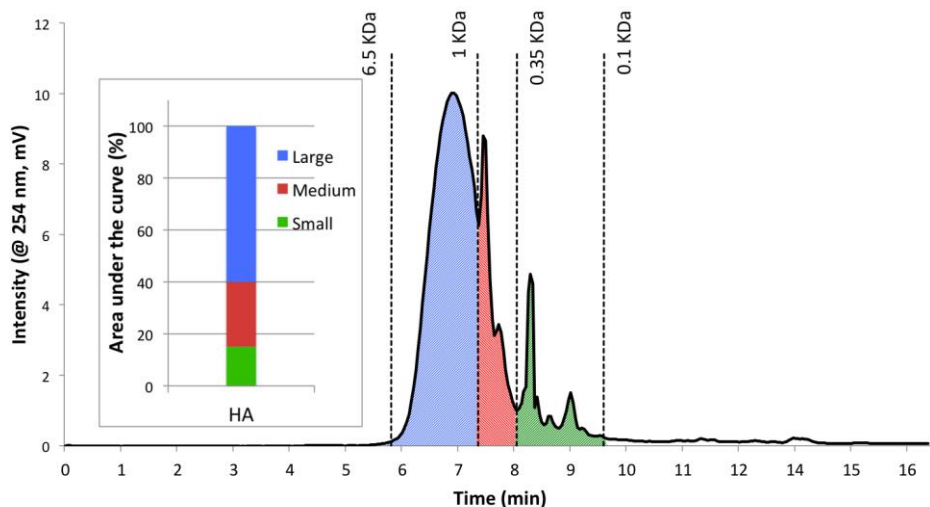
Fig 2. SEC chromatogram of HA complex (synthetic wastewater). The chromatogram is divided into three zones based on the main peaks: Large HA molecules (Blue), medium size HA molecules (Red) and small HA molecules (Green). The area under the curve was normalized and presented in the stacked column graph.
