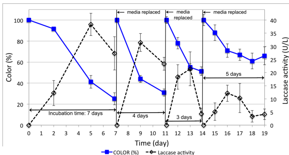
Fig 7. Color removal and laccase activity during the sequential batch experiment using immobilized fungi under non-sterile conditions. Results are presented as the average of duplicates and error bars indicate the min and max values.
