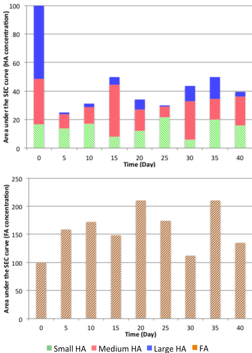
Fig 5. SEC analysis of the real wastewater during the fungal treatment. Top: HA, Bottom: FA. Results are presented as the average of at least duplicate measurements with standard deviation (for duplicates: range of min-max/2) of less than 2% for HA and less than 3% for FA.
