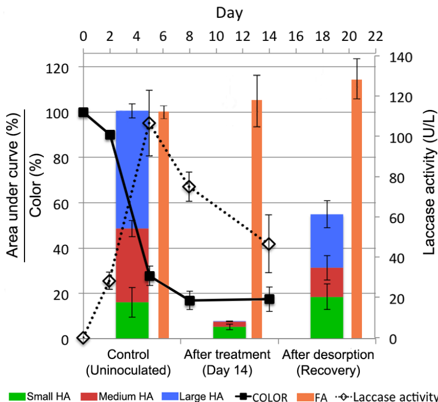
Fig 4. Fungal treatment of the real wastewater under sterile conditions. SEC results of HA and FA are presented as area under the curve (left Y-axis and lower X-axis). Color removal (%) and enzyme activity (laccase) were monitored during the incubation period (upper X axis). Results are presented as average of triplicates \pm SD.
