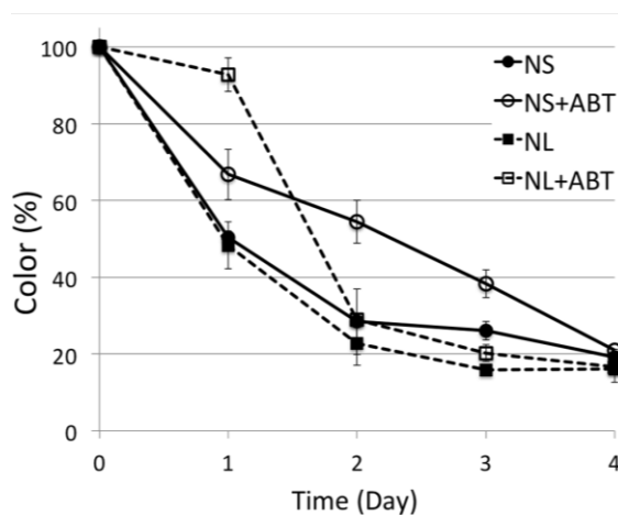
Fig 9. Role of CYP enzymes in HA bleaching by T. versicolor . ABT was used as the inhibitor of CYP enzymes.
