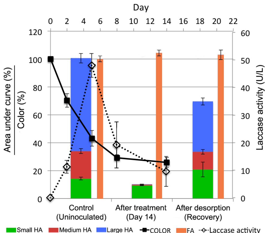
Fig 3. Fungal treatment of the synthetic wastewater under sterile conditions. SEC results of HA and FA are presented as area under the curve (left Y-axis and lower X-axis). Colour removal (%) and enzyme activity (laccase) were monitored during the incubation period (upper X axis). Results are presented as average of triplicates \pm SD.
