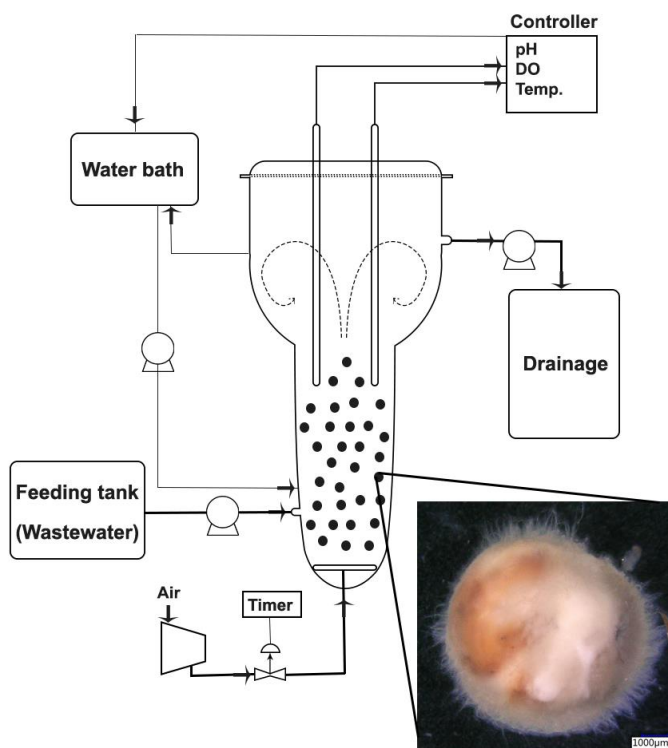
Fig 1. Schematic of the fluidized bed pulse aerated bioreactor setup inoculated with immobilized fungal granules
