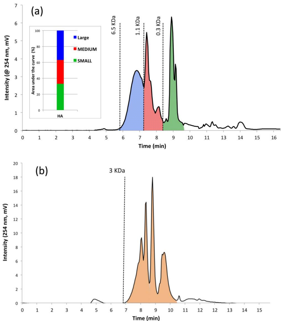
Fig 1. SEC chromatogram of HA (a) and FA (b) content of the wastewater
