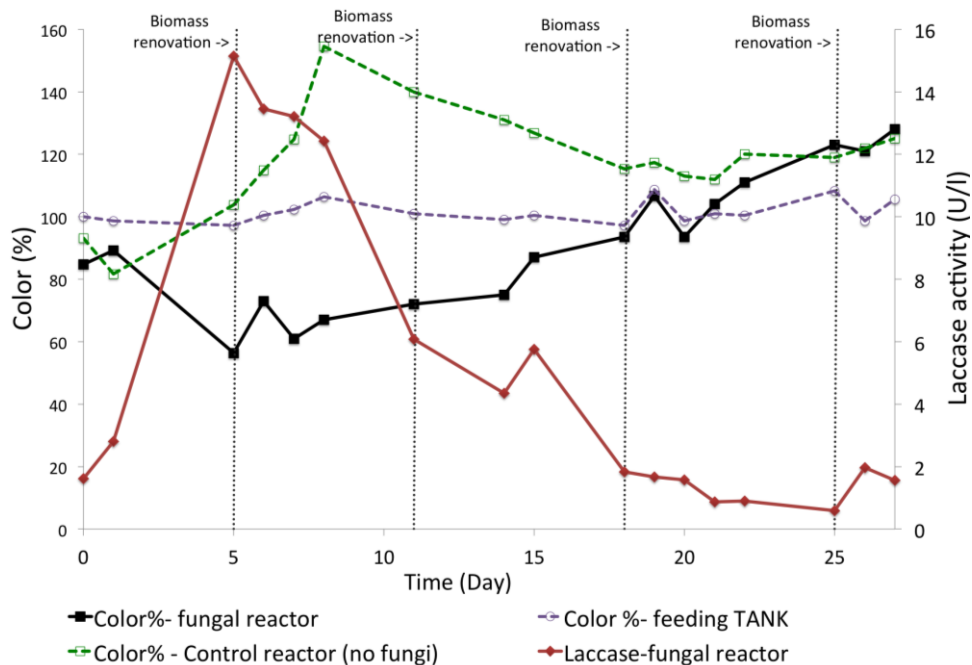
Fig 3. Evolution of the color in the fungal reactor (effluent), control reactor (without fungi) and the feeding tank (wastewater) in the treatment of real wastewater. Laccase activity in the fungal reactor is represented with rhombus. Vertical dotted lines mark instances of partial fungal biomass renewal. Time 0, is the inoculation time. The results are presented as the average of triplicate measurements, with standard error of less than 2% for color and less than 9% for laccase activity.
