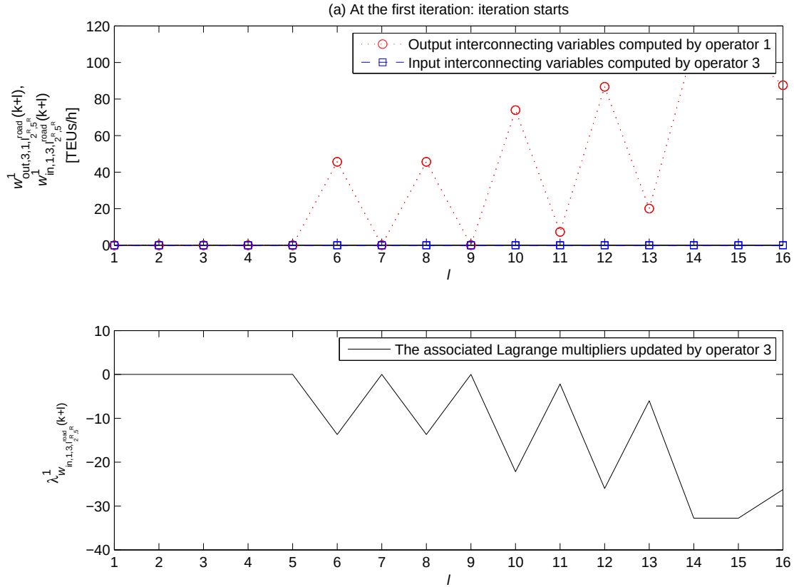
Figure 5.8: The coordination process on the values of interconnecting variables w^1_{out,3,1,l^{road}_{2R,5R}}(k+l) and w^1_{in,1,3,l^{road}_{2R,5R}}(k+l) over a prediction period of N_p = 16 time steps, hence, for l = 1, 2, \dots, 16 associated with the freeway link l^{road}_{2R,5R} between operator 1 and operator 3 at the first iteration of time step k = 1 in the parallel ALR-based DMPFC approach. The associated Lagrange multipliers \lambda^1_{w_{in,1,3,l^{road}_{2R,5R}}}(k+l) are shown in Figure 5.5(b).
