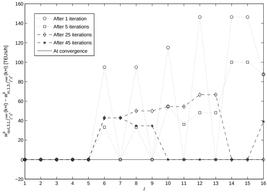
Figure 5.6: The evolution of the differences between the values of output interconnecting variable of the MPFC problem of operator 1, i.e., w_{out,3,1,l}^{road}(k+l) , and the values of the corresponding input interconnecting variable of the MPFC problem of operator 3, i.e., w_{in,1,3,l}^{road}(k+l) in the serial ALR-based DMPFC approach, for the time step k = 1 over a prediction period of N_p = 16 time steps, hence, for l = 1, 2, \dots, 16 .
