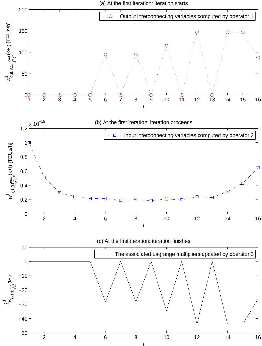
Figure 5.5: The coordination process on the values of interconnecting variables w_{out,3,1,l_{2R,5R}^{road}}^1(k+l) and w_{in,1,3,l_{2R,5R}^{road}}^1(k+l) over a prediction period of N_p = 16 time steps, hence, for l = 1, 2, \dots, 16 between operator 1 and operator 3 at the first iteration of time step k = 1 in the serial ALR-based DMPC approach. The associated Lagrange multipliers \lambda_{w_{in,1,3,l_{2R,5R}^{road}}^1(k+l)}^1 are shown in Figure 5.5(c).
