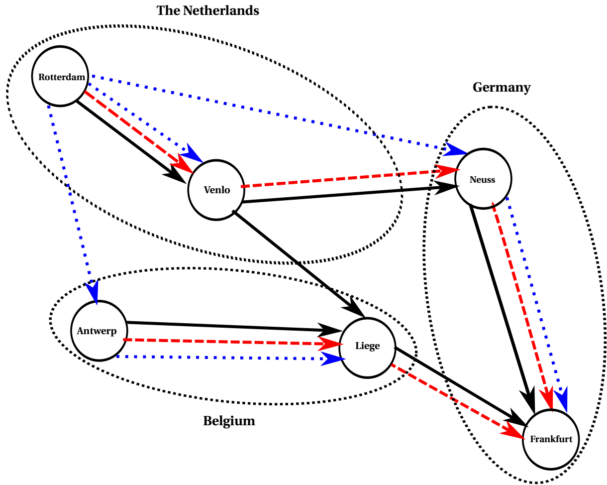
Figure 5.2: The topology of the multiple-region IFTN benchmark system between Rotterdam and Frankfurt. The solid black arcs, the dashed red arcs, and the dotted blue arcs indicate freeway links, railway links, and inland waterway links in the network, respectively.
