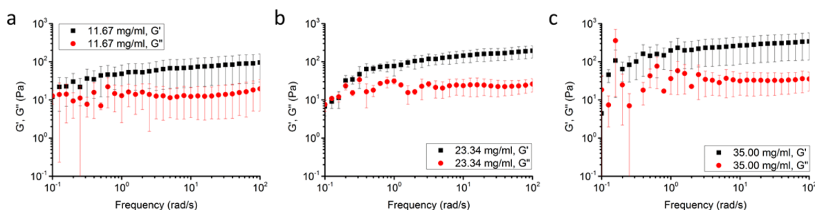
Figure 6. Frequency sweeps for PS- b -PEO fibril micellar solutions with different concentrations at 90 °C: (a) 11.67, (b) 23.34, and (c) 35.00 mg/mL. Rheometer in plate-plate geometry with a gap of 200 \mu m and 0.05% applied strain.
