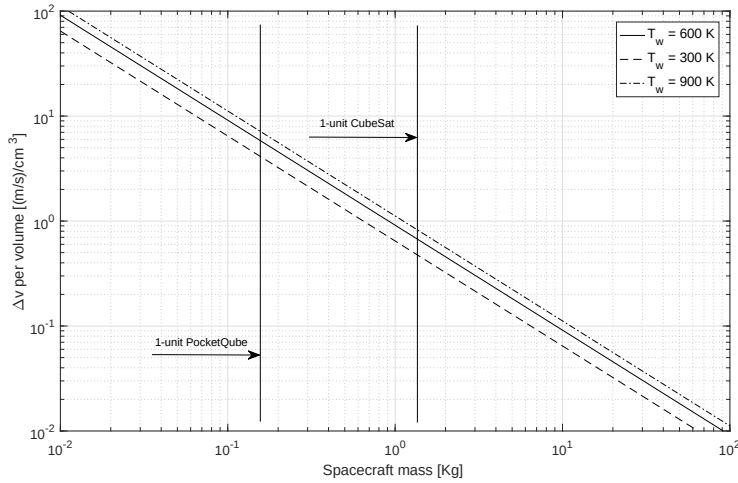
Figure 6.4: Relation between the Delta-V per volume of fluid and the spacecraft mass.
