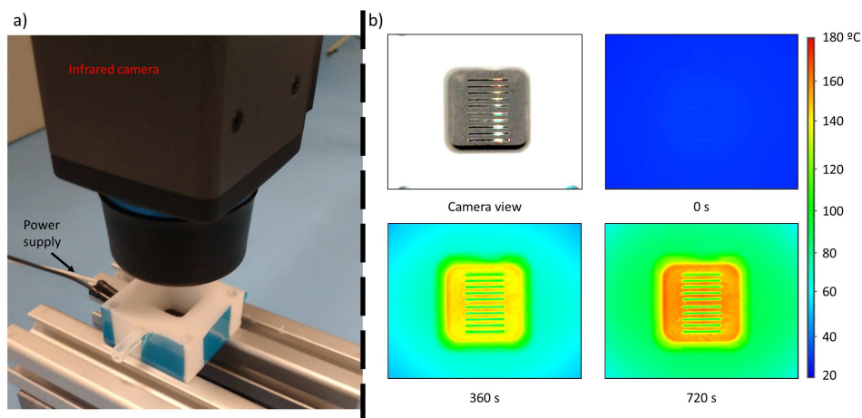
Figure 5.5: a) Setup used to define the temperature coefficient of the resistance ( \beta ) in Equation 5.2. b) The temperature measurement of the chip surface using an infrared camera. The left top side shows the camera view; the chip is painted with graphite ink that provides an uniform emissivity of 0.97. The other images are from the infrared camera at different moments after applying a constant voltage of 39 V.
