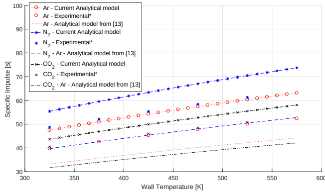
Figure 4.5: Specific impulse as a function of T_w for different propellants and constant mass flow rate. *The experimental results were plotted from the fit equations presented in Ketsdever et al. (2005).
