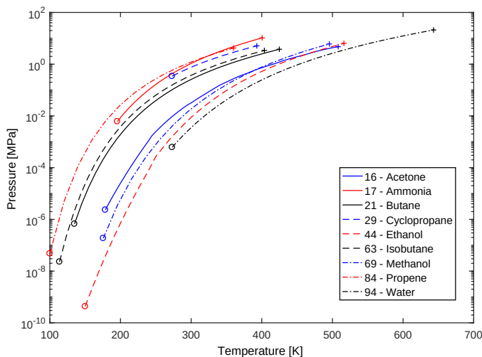
Figure 2.3: Saturation curve. ^{\circ} denotes the triple point and ^{+} denotes the critical point. The fluid is liquid on the left side of the curve, and gaseous on its right side.
