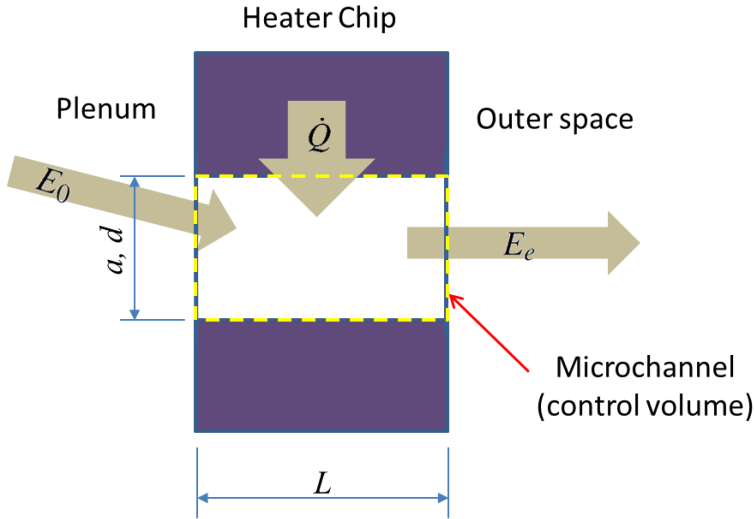
Figure 4.1: Balance of energy inside the microchannel where E_0 is the energy which gets in the control volume, E_e is the energy which gets out the control volume and \dot{Q} is the heat transferred to the gas inside the control volume.
