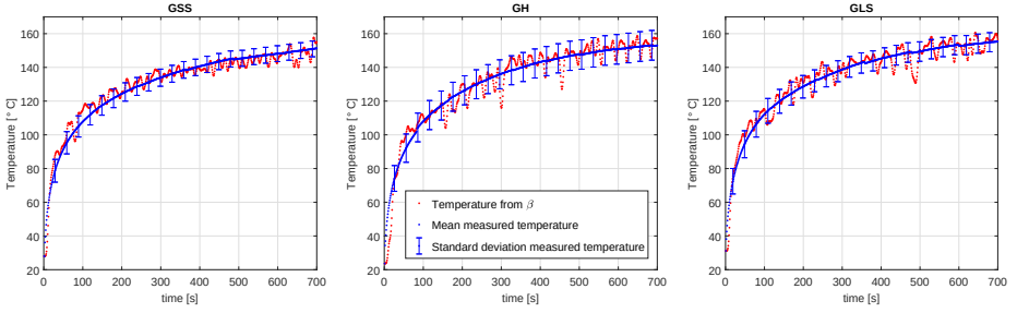
Figure 5.10: Comparison between the temperature measurement from the infrared camera and the calculated temperature based on Equation 5.2.
