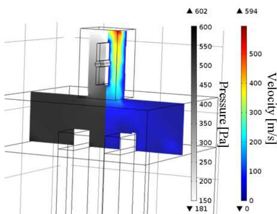
Figure B.4: Velocity and pressure field of the steam from the tank to plenum. Left hand side (Greyscale) pressure field, right hand side (Coloured) velocity field.
