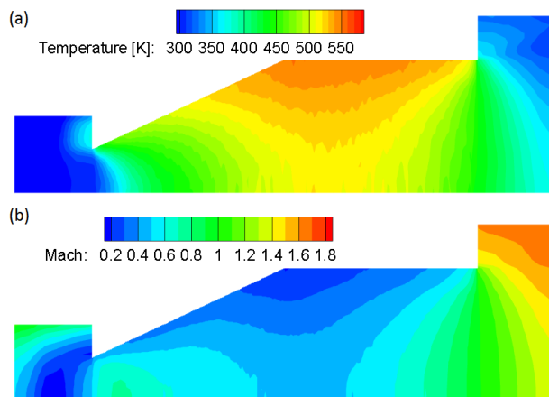
Figure 3.17: Temperature (a) and Mach number (b) maps for the first-half divergent microchannel (case 4), for a divergent angle of 25 degrees, plenum pressure of 150 Pa and wall temperature of 573 K.
