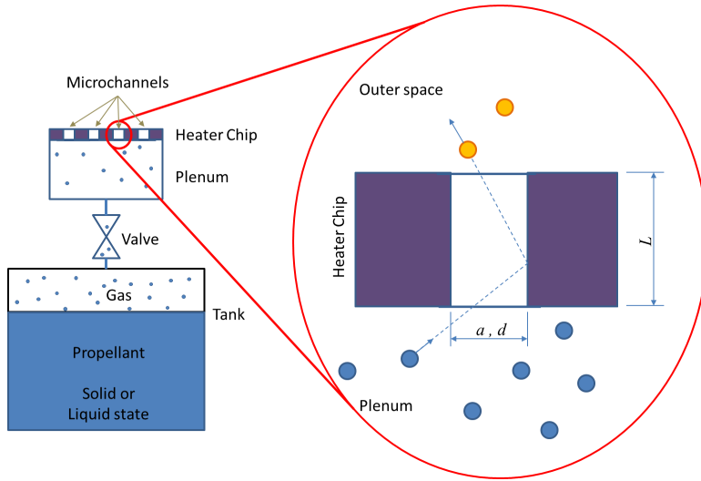
Figure 1.5: Schematic of the LPM. Left: the complete system composed by tank, feed system and thruster. Right: The detailed microchannel and the particles behavior.
