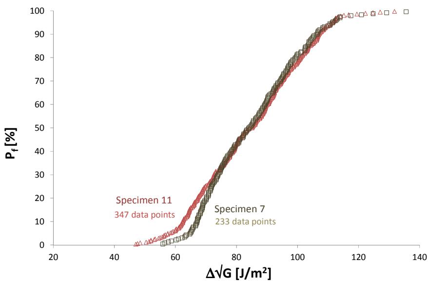
Figure 8. Comparison between the cumulative density functions at da/dN = 4.5 \cdot 10^{-7} m/cycle for the curves in Figure 5 and Figure 6
