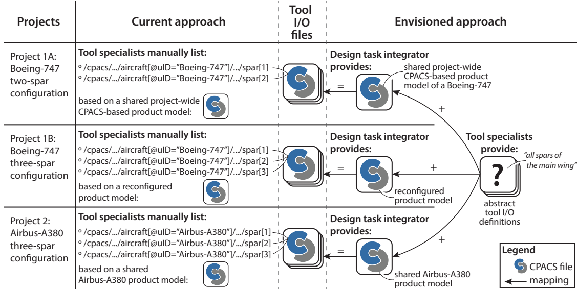
Fig. 11 Visual explanation of the current approach for defining tool I/O files and the envisioned approach for a more flexible definition using a baseline file mapping
