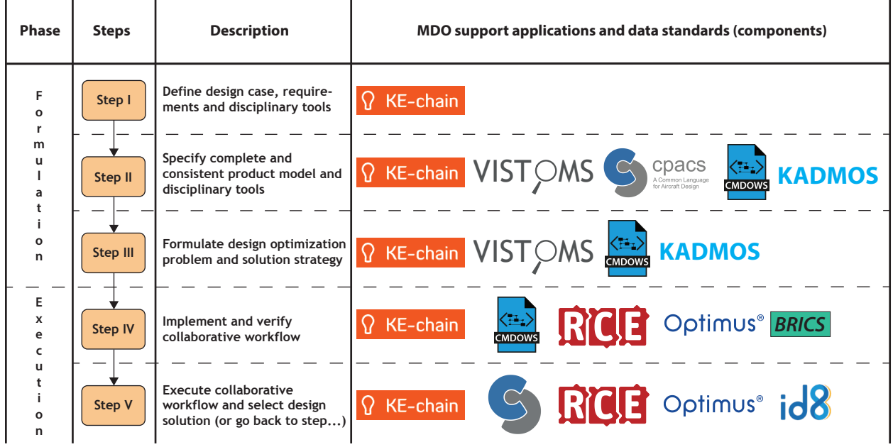
Fig. 1 AGILE five-step development process (adapted from earlier work[5])
