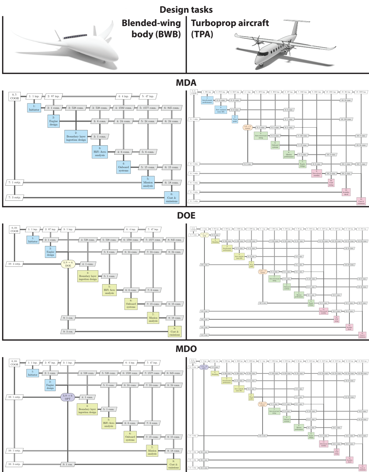
Fig. 5 Snapshots of the XDSMs of the formulated workflows for the BWB and TPA design tasks. Each XDSM corresponds to a CMDOWS file (C3) containing the neutral definition of the MDO solution strategy.
