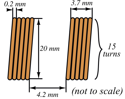
Fig. 17. Nominal geometric specifications of the fabricated link coils. Both coils are circular, identical, and coaxially aligned.
