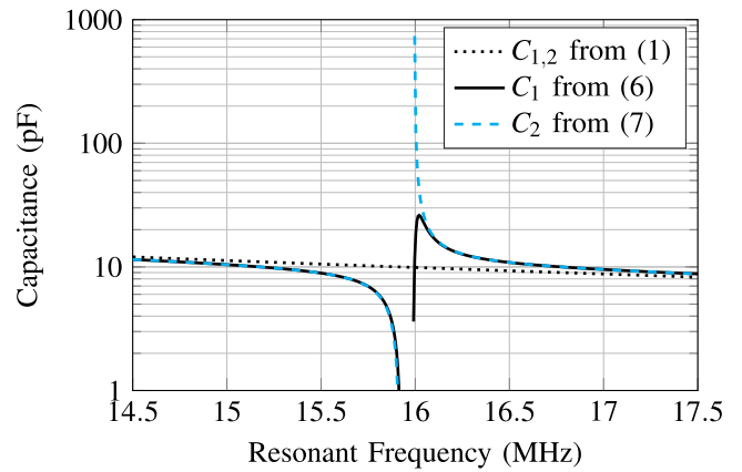
Fig. 6. Determining capacitance through resonant frequency.
