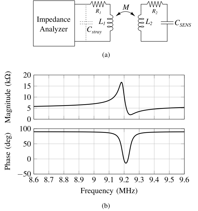
Fig. 2. The phase-dip measurement approach for wireless capacitive sensing. L_1 = 10 \mu\text{H} , L_2 = 100 \mu\text{H} , R_{1,2} = 2 \Omega , M = 3.162 \mu\text{H} , C_{SENS} = 3 \text{ pF} . (a) Phase-dip measurement setup. (b) Example link impedance measurement.
