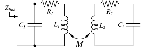
Fig. 3. General case inductive link model.
