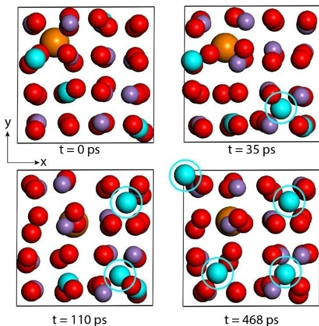
Figure 6.13: Snapshots of the P – \text{Na}_{0.125}\text{Mn}_2\text{O}_4 structure throughout the 500 ps MD simulation at 600 K: (top-left) only Na occupies a tetrahedral position; (bottom-right) all 4 Ni occupy tetrahedral positions
