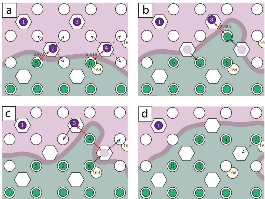
Figure A1: Time lapse that depicts the Li-ion reaction mechanisms as viewed from the xz plane of a small part of the 2x1x2 supercell at the first ps of the MD simulation, dashed lines indicate the possibility of hop while the solid line the hop that actually occurs. The red line reflects the type 1 interface configurations presented in the report
