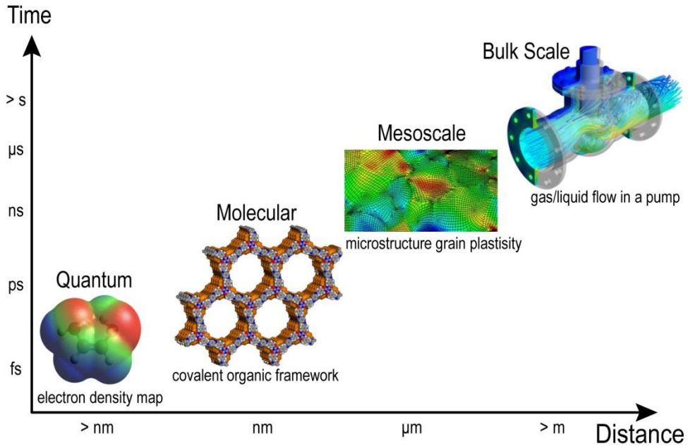
Figure 1.6: Classification of computational models with respect to the lengthscales and timescales.
