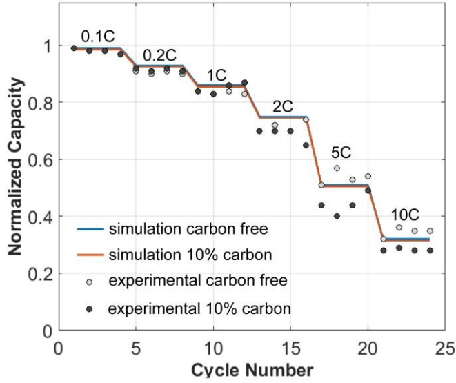
Figure 4.11: Comparison between experimental (dots) 61 and the simulated (line) capacities for the battery reported by Kim et al. 61
