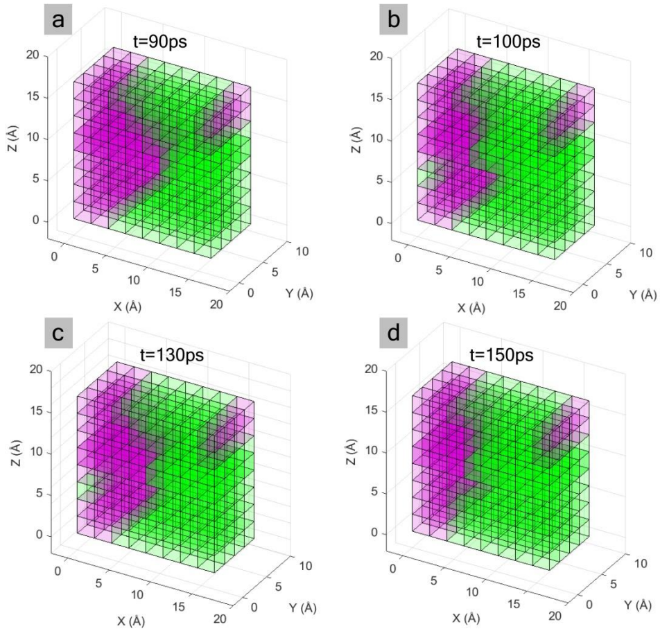
Figure 3.10: Time lapse after the interface equilibration in the 2x1x2 supercell at 520K that depicts the slight changes after the equilibration period (90 to 100ps). It should be realized that the DFT calculations are performed under periodic boundary conditions.
